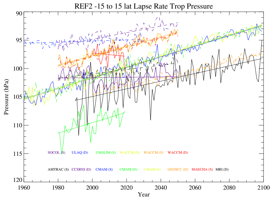
Fig. 11. Tropical mean Lapse Rate Tropopause Pressure from various models showing expected future scenarios (REF2). Thin lines are linear trends. Models are either solid (S) or dashed (D) lines as indicated in the legend.
