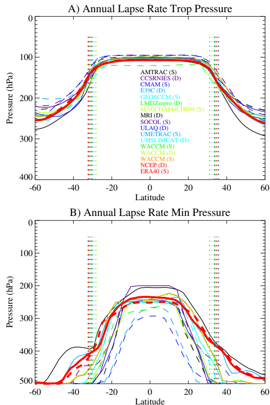
Fig. 3. Zonal mean (A) Lapse Rate Tropopause Pressure and (B) Lapse Rate Minimum Pressure from CCMVal models (REF1 scenarios, 1980–2005). Vertical Dotted lines are meridional tropopause edges. Thick Red lines are NCEP/NCAR (dashed) and ERA40 (solid) Reanalyses. Models are either solid (S) or dashed (D) lines as indicated in the legend in (A).
