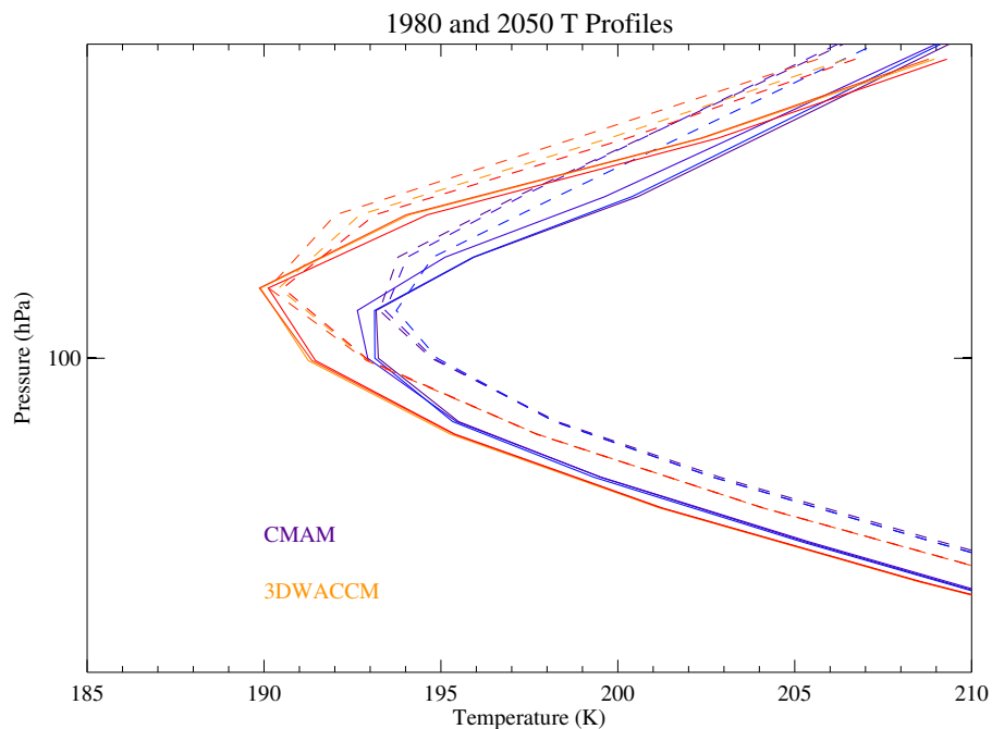
Fig. 15. Tropical temperature profiles from WACCM and CMAM models for future (REF2) scenarios. Solid lines: 1980 average. Dashed lines: 2050 average for each of 3 realizations.
