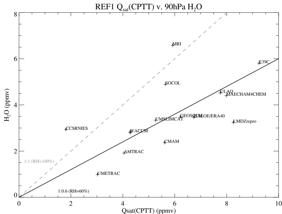
Fig. 16. Scatterplot of Saturation Vapor Mixing Ratio of the Cold Point Tropopause Temperature, Q_{\text{sat}}(\text{CPTT}) and the 90 hPa tropical water vapor mixing ratio for each historical (REF1) run, as well as using ERA40 temperatures and HALOE 100hPa water vapor (ERA40/HALOE). Gray dashed line is 1:1 line (100% RH), Black solid line is 1:0.6 (60% RH).
