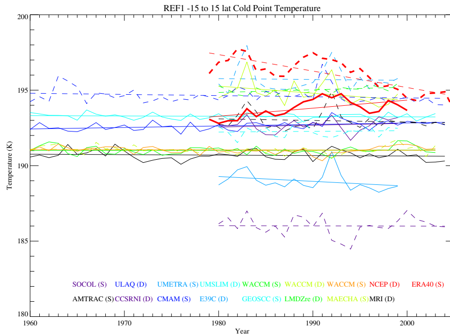
Fig. 4. Tropical mean Cold Point Tropopause Temperature from various models for Historical (REF1) runs. Thin lines are linear trends. Models are either solid (S) or dashed (D) lines as indicated in the legend. Thick Red lines are NCEP/NCAR (dashed) and ERA40 (solid) Reanalyses.
