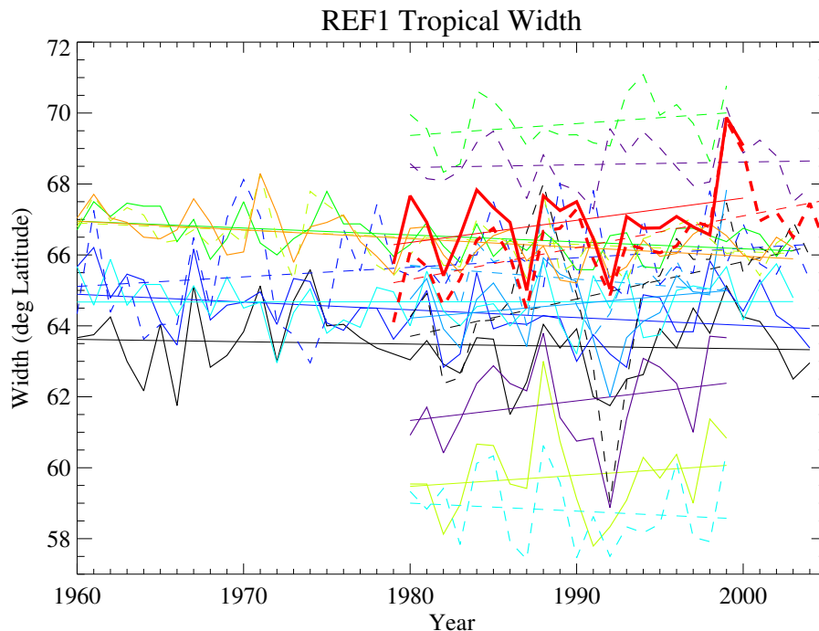
Fig. 9. Tropical mean TTL width (in latitude) models for historical (REF1) scenarios. Thin lines are linear trends. Models are either solid (S) or dashed (D) lines as indicated in the legend for Fig. 8. Thick Red lines are NCEP/NCAR (dashed) and ERA40 (solid) Reanalyses.
