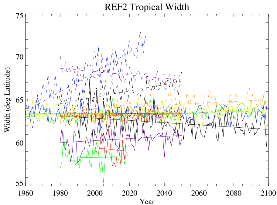
Fig. 14. Tropical mean TTL width (in latitude) models for future (REF2) scenarios. Thin lines are linear trends. Models are either solid (S) or dashed (D) lines as indicated in the legend for Fig. 12.
