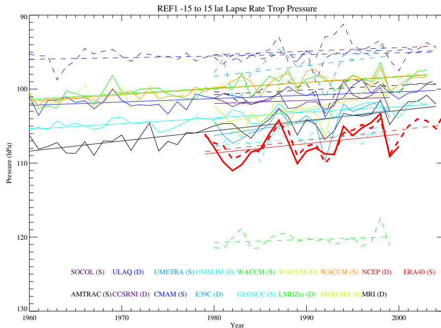
Fig. 5. Tropical mean Lapse Rate Tropopause Pressure from various models for Historical (REF1) runs. Thin lines are linear trends. Models are either solid (S) or dashed (D) lines as indicated in the legend. Thick Red lines are NCEP/NCAR (dashed) and ERA40 (solid) Reanalyses.
