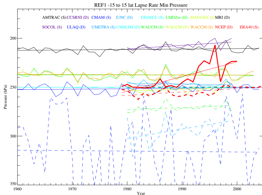
Fig. 6. Tropical mean Lapse Rate Minimum Pressure from various models for Historical (REF1) runs. Thin lines are linear trends. Models are either solid (S) or dashed (D) lines as indicated in the legend. Thick Red lines are NCEP/NCAR (dashed) and ERA40 (solid) Reanalyses.
