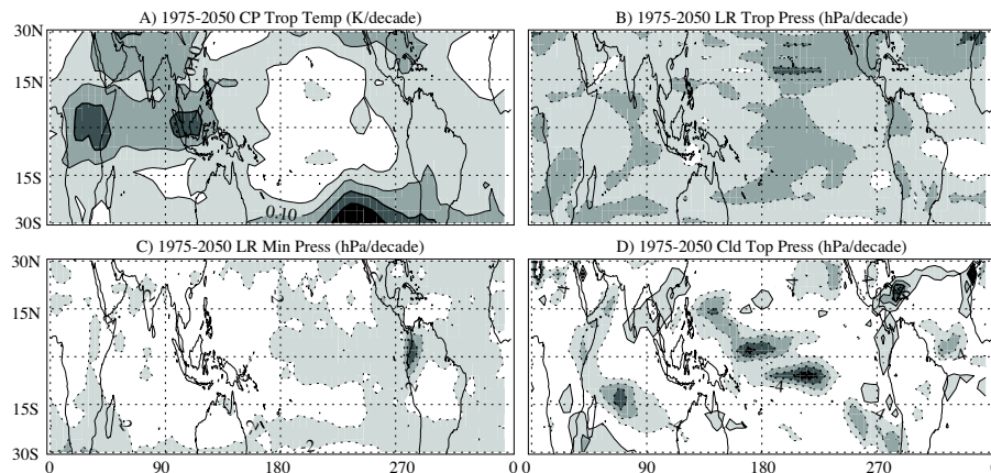
Fig. 13. Map of trends from future (REF2) WACCM simulations. (A) Cold Point Tropopause Temperature trends, contour interval 0.05 K/decade. (B) Lapse Rate Tropopause pressure trends, contour interval 0.5 hPa/decade (C) Lapse Rate Minimum Pressure trends, contour interval 2 hPa/decade. (D) Cloud Top Pressure trends, contour interval 2 hPa/decade. Dashed lines are negative trends, no zero line.
