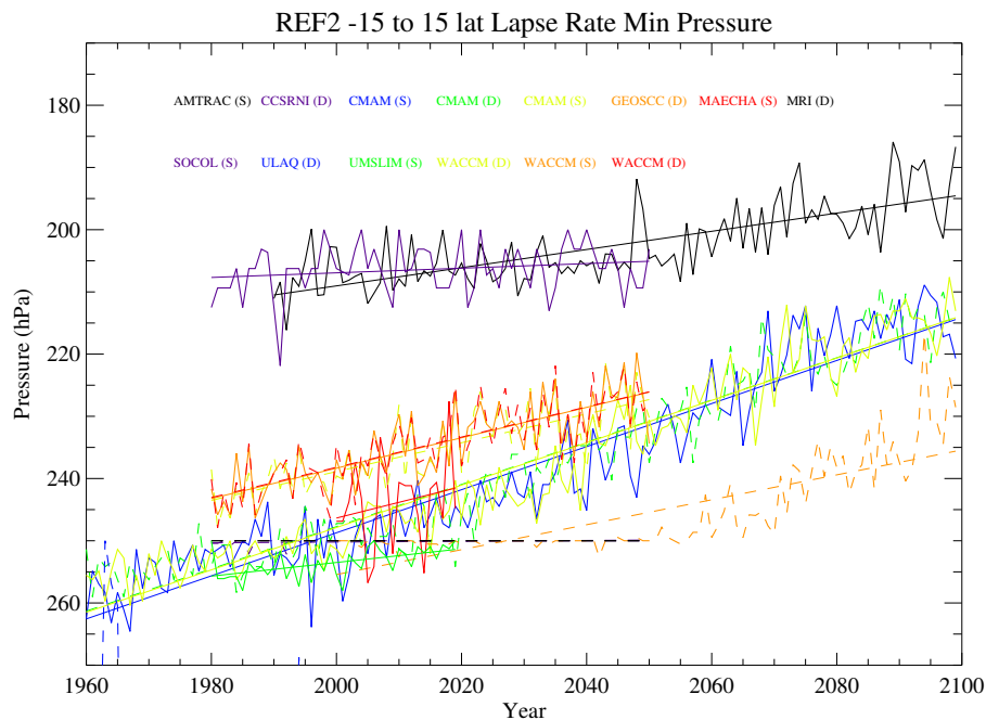
Fig. 12. Tropical mean Lapse Rate Minimum Pressure from various models showing expected future scenarios (REF2). Thin lines are linear trends. Models are either solid (S) or dashed (D) lines as indicated in the legend. Note that ULAQ is off scale.
