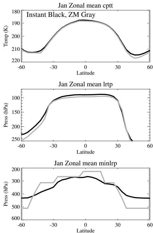
Fig. 1. Comparison between TTL diagnostics calculated using instantaneous 3-D output (Black) and zonal mean monthly output (Gray) for Cold Point tropopause temperature (top), lapse rate tropopause pressure (middle) and lapse rate minimum pressure (bottom).
