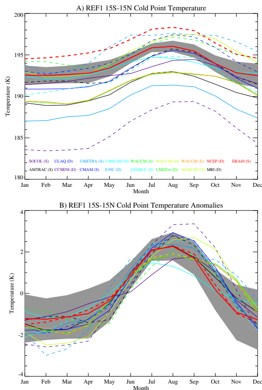
Fig. 2. Annual Cycle of Tropical (15S–15N) Zonal mean Cold point Temperature from REF1 (1980–2005) scenarios of CCMVal Models. (A) Temperature. (B) Temperature anomalies (annual mean removed). Thick Red lines are NCEP/NCAR (dotted) and ERA40 (solid) Reanalysis. Gray shading is \pm 2 standard deviations from ERA40. Models are either solid (S) or dashed (D) lines as indicated in the legend.
