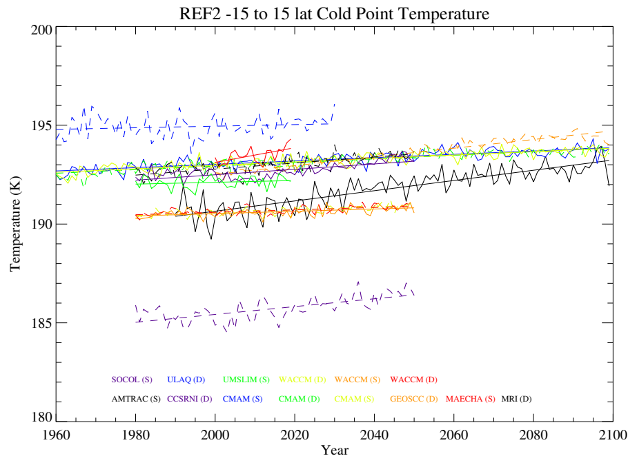
Fig. 10. Tropical mean Cold Point Tropopause Temperature from various models showing expected future scenarios (REF2). Thin lines are linear trends. Models are either solid (S) or dashed (D) lines as indicated in the legend.
