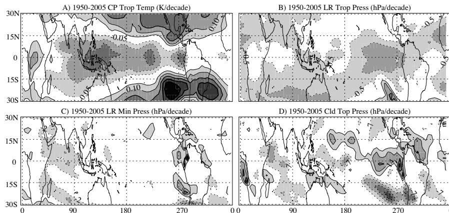
Fig. 7. Map of trends from historical (REF1) WACCM simulations. (A) Cold Point Tropopause Temperature trends, contour interval 0.05 K/decade. (B) Lapse Rate Tropopause pressure trends, contour interval 0.5 hPa/decade (C) Lapse Rate Minimum Pressure trends, contour interval 2 hPa/decade. (D) Cloud Top Pressure trends, contour interval 7 hPa/decade. Dashed lines are negative trends, no zero line.
