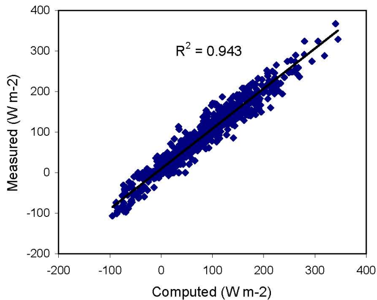
Fig. 5. Correlation diagram for variational calculated and measured heat flux.
