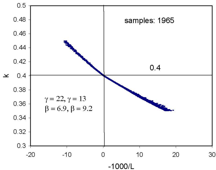
Fig. 3. Same as Fig. 2 except for the profile constants (\gamma_m, \gamma_h, \beta_m, \beta_h) = (22, 13, 6.9, 9.2) .
