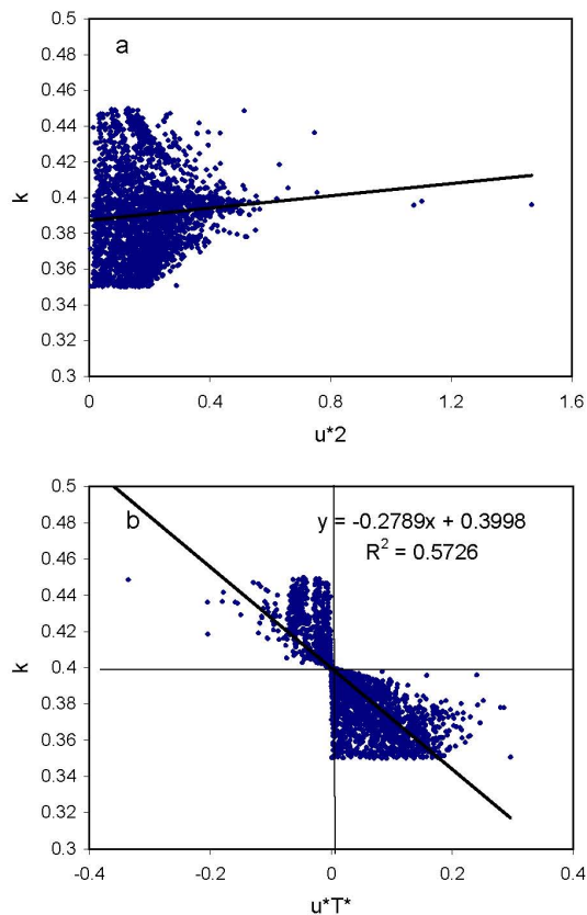
Fig. 4. Variation of \kappa with (a) momentum flux u_*^2 (m 2 s -2 ) and (b) heat flux u_* T_* (m s -1 K). Linear equations of fitting line are also displayed. R^2 is the coefficient of determination.
