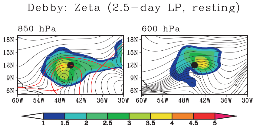
Fig. 8. Streamlines of horizontal flow at (a) 850 hPa and (b) 600 hPa at the genesis time of Hurricane Debby, in the resting frame. Shading indicates relative vorticity (units: 10^{-5} \text{ s}^{-1} ) which is invariant with respect to translation, therefore identical in translating and resting frames (cp. final panels of Figs. 6 and 7).
