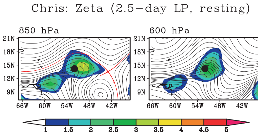
Fig. 13. Streamlines of horizontal flow at (a) 850 hPa and (b) 600 hPa at the genesis time of Tropical Storm Chris, in the resting frame. Shading indicates relative vorticity (units: 10^{-5} \text{ s}^{-1} ) which is invariant with respect to translation, therefore identical in translating and resting frames (cp. final panel of Fig. 11).
