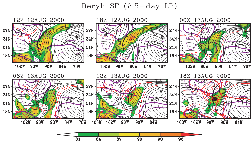
Fig. 19. Streamlines of horizontal flow at 850 hPa for the genesis sequence of Tropical Storm Beryl as in Fig. 16, with high values of ERA-40 saturation fraction indicated by shading (units: percent). The sequence of frames translates westward at the zonal propagation speed of the parent wave at 850 hPa ( -3.8 \pm 2.8 \text{ ms}^{-1} ) and streamlines are displayed in this gauge.
