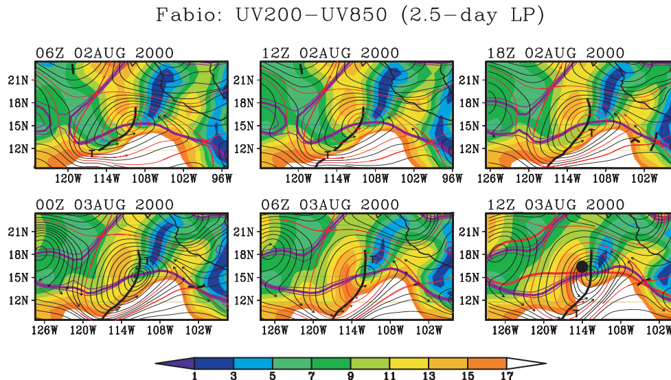
Fig. 26. Streamlines of horizontal flow at 600 hPa for the genesis sequence of Tropical Storm Fabio as in Fig. 22, with ERA-40 850–200 hPa vertical shear (magnitude of shear vector, units: \text{ms}^{-1} ) indicated by shading. The sequence of frames translates westward at the zonal propagation speed of the parent wave at 600 hPa ( -3.1 \pm 0.8 \text{ ms}^{-1} ) and streamlines are displayed in this gauge.
