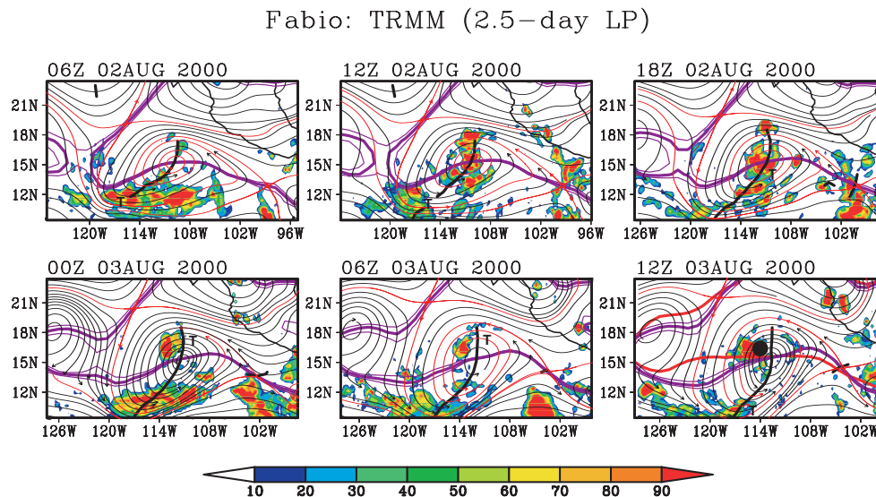
Fig. 24. Streamlines of horizontal flow at 600 hPa for the genesis sequence of Tropical Storm Fabio as in Fig. 22, with high values of TRMM 3-h accumulated precipitation indicated by shading (units: mm/day). The sequence of frames translates westward at the zonal propagation speed of the parent wave at 600 hPa ( -3.1 \pm 0.8 \text{ ms}^{-1} ) and streamlines are displayed in this gauge.
