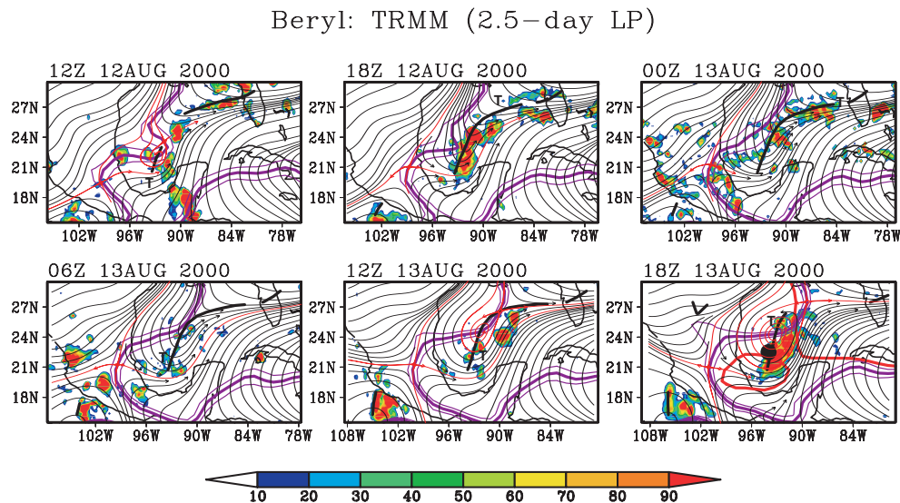
Fig. 20. Streamlines of horizontal flow at 600 hPa for the genesis sequence of Tropical Storm Beryl as in Fig. 17, with high values of TRMM 3-h accumulated precipitation indicated by shading (units: mm/day). The sequence of frames translates westward at the zonal propagation speed of the parent wave at 600 hPa ( -3.1 \pm 0.8 \text{ ms}^{-1} ) and streamlines are displayed in this gauge.
