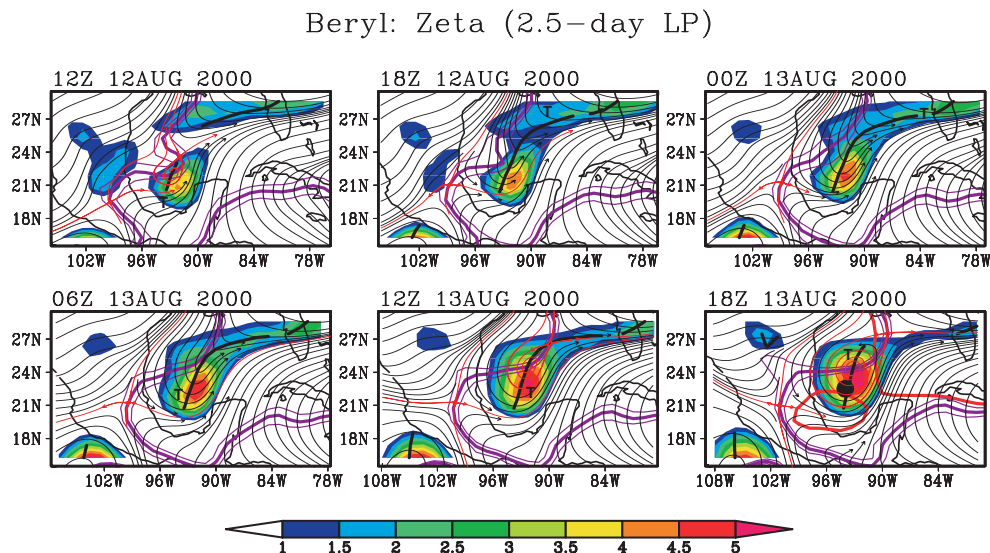
Fig. 17. Streamlines of horizontal flow for the genesis sequence of Tropical Storm Beryl as in Fig. 16, but at 600 hPa. Shading indicates relative vorticity (units: 10^{-5} \text{ s}^{-1} ). The sequence of frames translates westward at the zonal propagation speed of the parent wave at 600 hPa ( -3.1 \pm 0.8 \text{ ms}^{-1} ) and streamlines are displayed in this gauge.
