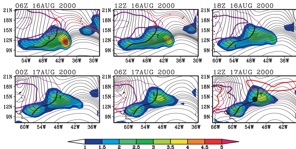
Fig. 11. Streamlines of horizontal (rotational + divergent) flow at 850 hPa, as seen in ERA-40 data, for six consecutive analyses leading up to the best-track genesis time of Tropical Storm Chris (2000). Streamlines passing near a separatrix are shown in red. Shading indicates relative vorticity (units: 10^{-5} \text{ s}^{-1} ). The sequence of frames translates westward at the zonal propagation speed of the parent wave at 850 hPa as estimated from the Hovmöller method ( -9.1 \pm 1.1 \text{ ms}^{-1} ) and streamlines are displayed in this gauge; note that relative vorticity itself is invariant with respect to the translation. Isopleths of zero relative zonal flow are shown (purple) together with their uncertainty. In the final panel of the sequence the critical latitude of the parent wave is also indicated (red) corresponding to isopleths of zero relative zonal flow in low-frequency data with periods longer than 9 days. The wave's trough axis is shown for reference (black). The genesis location is indicated by the black dot in the final panel.
