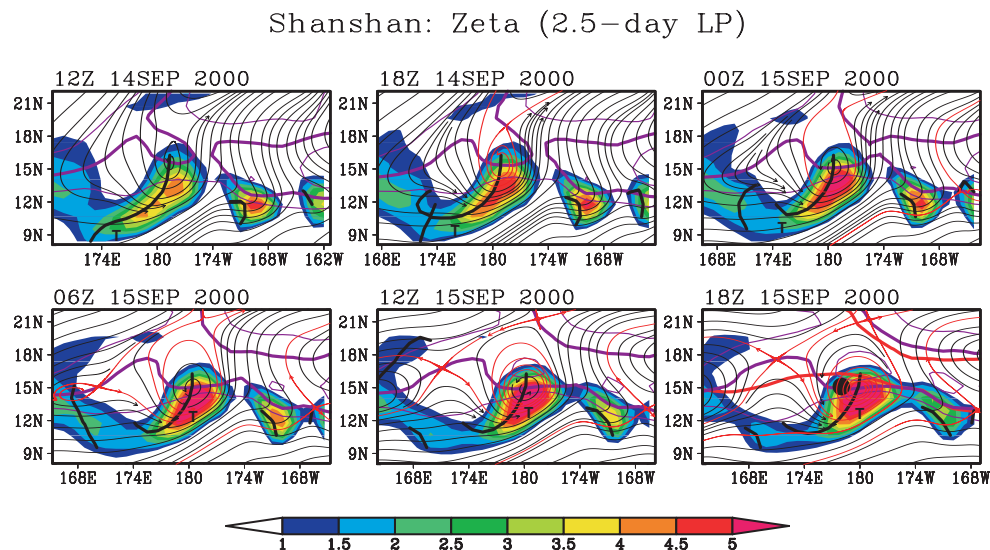
Fig. 28. Streamlines of horizontal flow for the genesis sequence of Super Typhoon Shanshan as in Fig. 27, but at 600 hPa. Shading indicates relative vorticity (units: 10^{-5} \text{ s}^{-1} ). The sequence of frames translates westward at the zonal propagation speed of the parent wave at 600 hPa ( -5.7 \pm 2.8 \text{ ms}^{-1} ) and streamlines are displayed in this gauge.
