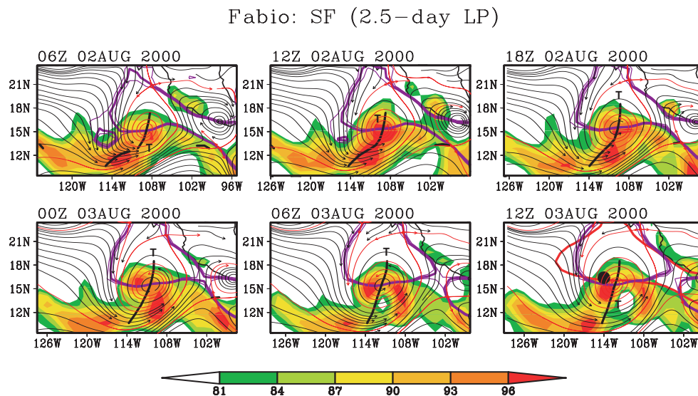
Fig. 23. Streamlines of horizontal flow at 850 hPa for the genesis sequence of Tropical Storm Fabio as in Fig. 21, with high values of ERA-40 saturation fraction indicated by shading (units: percent). The sequence of frames translates westward at the zonal propagation speed of the parent wave at 850 hPa ( -3.7 \pm 0.5 \text{ ms}^{-1} ) and streamlines are displayed in this gauge.
