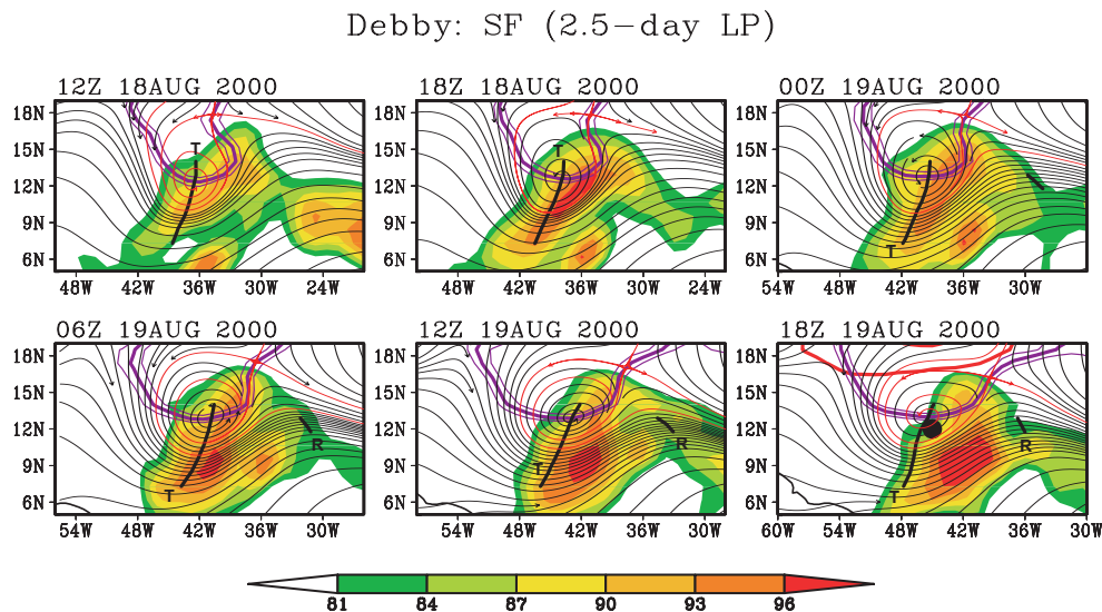
Fig. 9. Streamlines of horizontal flow at 850 hPa for the genesis sequence of Hurricane Debby as in Fig. 6, with high values of ERA-40 saturation fraction indicated by shading (units: percent). The sequence of frames translates westward at the zonal propagation speed of the parent wave at 850 hPa ( -10.0 \pm 0.6 \text{ ms}^{-1} ) and streamlines are displayed in this gauge.
