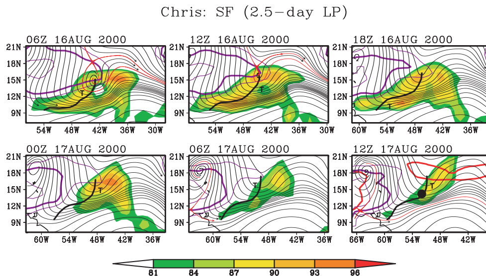
Fig. 14. Streamlines of horizontal flow at 850 hPa for the genesis sequence of Tropical Storm Chris as in Fig. 11, with high values of ERA-40 saturation fraction indicated by shading (units: percent). The sequence of frames translates westward at the zonal propagation speed of the parent wave at 850 hPa ( -9.1 \pm 1.1 \text{ ms}^{-1} ) and streamlines are displayed in this gauge.
