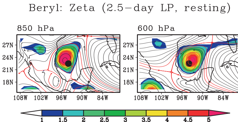
Fig. 18. Streamlines of horizontal flow at (a) 850 hPa and (b) 600 hPa at the genesis time of Tropical Storm Beryl, in the resting frame. Shading indicates relative vorticity (units: 10^{-5} \text{ s}^{-1} ) which is invariant with respect to translation, therefore identical in translating and resting frames (cp. final panels of Figs. 16 and 17).
