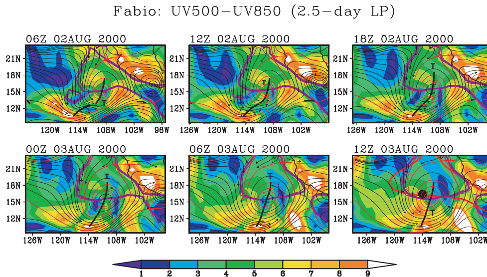
Fig. 25. Streamlines of horizontal flow at 850 hPa for the genesis sequence of Tropical Storm Fabio as in Fig. 21, with ERA-40 850–500 hPa vertical shear (magnitude of shear vector, units: \text{ms}^{-1} ) indicated by shading. The sequence of frames translates westward at the zonal propagation speed of the parent wave at 850 hPa ( -3.7 \pm 0.5 \text{ ms}^{-1} ) and streamlines are displayed in this gauge.
