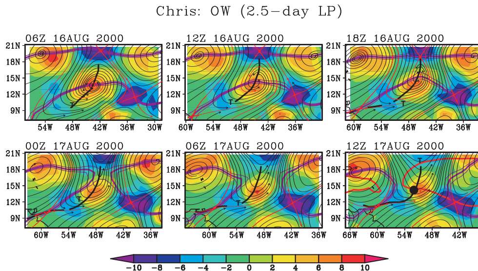
Fig. 12. Streamlines of horizontal flow for the genesis sequence of Tropical Storm Chris as in Fig. 11, but at 600 hPa. Shading indicates the Okubo-Weiss parameter (units: 10^{-10} \text{s}^{-2} ) as defined in Eq. (1). This quantity, like vorticity, is invariant with respect to translation, therefore identical in translating and resting frames. The sequence of frames translates westward at the zonal propagation speed of the parent wave at 600 hPa ( -8.5 \pm 0.5 \text{ms}^{-1} ) and streamlines are displayed in this gauge.
