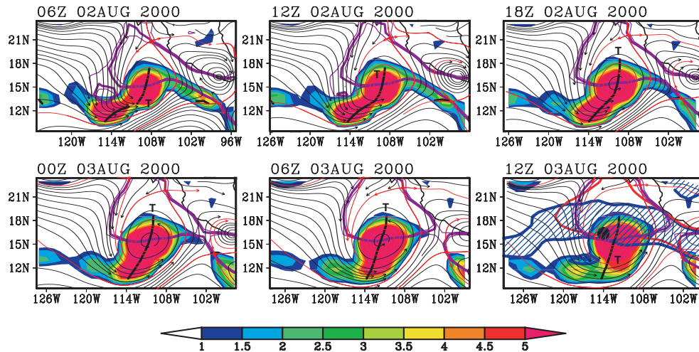
Fig. 21. Streamlines of horizontal (rotational + divergent) flow at 850 hPa, as seen in ERA-40 data, for six consecutive analyses leading up to the best-track genesis time of Tropical Storm Fabio (2000). Streamlines passing near a separatrix are shown in red. Shading indicates relative vorticity (units: 10^{-5} \text{ s}^{-1} ). The sequence of frames translates westward at the zonal propagation speed of the parent wave at 850 hPa as estimated from the Hovmöller method ( -3.7 \pm 0.5 \text{ ms}^{-1} ) and streamlines are displayed in this gauge; note that relative vorticity itself is invariant with respect to the translation. Isopleths of zero relative zonal flow are shown (purple) together with their uncertainty. In the final panel of the sequence the critical latitude of the parent wave is also indicated (red) corresponding to isopleths of zero relative zonal flow in low-frequency data with periods longer than 9 days. These data were also used to estimate the zero contour of absolute vorticity gradient or “effective \beta ” (blue). This quantity is negative in the zone just north of the genesis latitude, bracketed by the blue curves (diagonal hatching). The wave’s trough axis is shown for reference (black). The genesis location is indicated by the black dot in the final panel.
