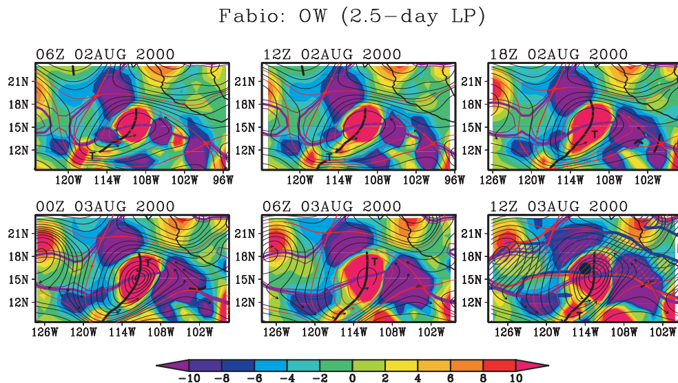
Fig. 22. Streamlines of horizontal flow for the genesis sequence of Tropical Storm Fabio as in Fig. 21, but at 600 hPa. Shading indicates the Okubo-Weiss parameter (units: 10^{-10} \text{ s}^{-2} ) as defined in Eq. (1). This quantity, like vorticity, is invariant with respect to translation, therefore identical in translating and resting frames. The sequence of frames translates westward at the zonal propagation speed of the parent wave at 600 hPa ( -3.1 \pm 0.8 \text{ ms}^{-1} ) and streamlines are displayed in this gauge. Red and blue lines in the final panel show the wave's critical latitude and isopleth of zero effective \beta as estimated from low-frequency data with periods longer than 9 days.
