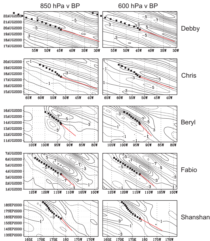
Fig. 5. Hovmöller plots of band-pass meridional velocity component at 850 hPa (left column) and 600 hPa (right column) in a longitude-time plane for the five cases of summer 2000 high-latitude tropical cyclones: (a) Hurricane Debby; (b) Tropical Storm Chris; (c) Tropical Storm Beryl; (d) Tropical Storm Fabio; (e) Super Typhoon Shanshan. Black circles indicate the best-track longitude and time of genesis, while black squares indicate subsequent best track locations at 6-h intervals. Red line denotes the Hovmöller estimate of zonal translation speed C_p .
