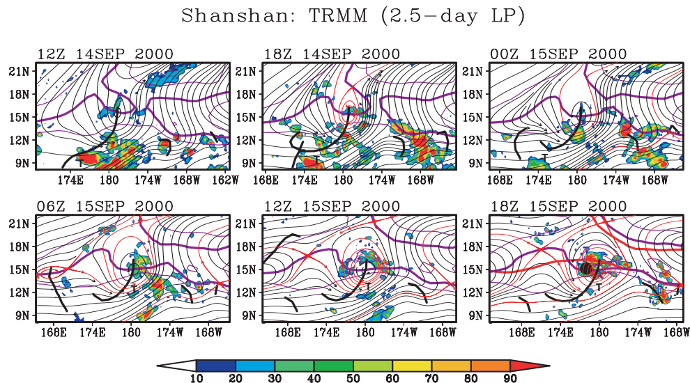
Fig. 30. Streamlines of horizontal flow at 600 hPa for the genesis sequence of Super Typhoon Shanshan as in Fig. 27, with high values of TRMM 3-h accumulated precipitation indicated by shading. Units: mm/day. The sequence of frames translates westward at the zonal propagation speed of the parent wave at 600 hPa ( -5.7 \pm 2.8 \text{ ms}^{-1} ) and streamlines are displayed in this gauge.
