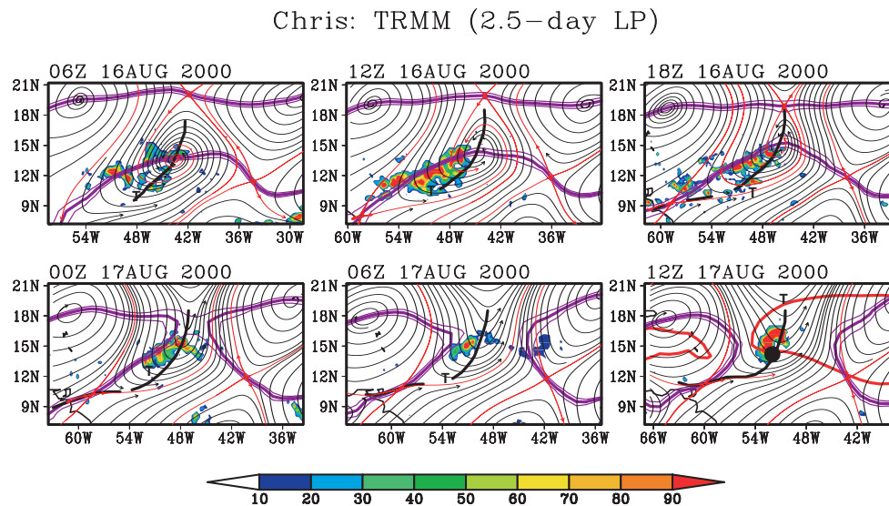
Fig. 15. Streamlines of horizontal flow at 600 hPa for the genesis sequence of Tropical Storm Chris as in Fig. 12, with high values of TRMM 3-h accumulated precipitation indicated by shading (units: mm/day). The sequence of frames translates westward at the zonal propagation speed of the parent wave at 600 hPa ( -8.5 \pm 0.5 \text{ ms}^{-1} ) and streamlines are displayed in this gauge.
