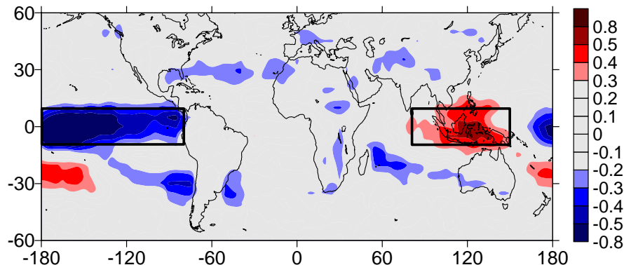
Fig. 5. Correlation coefficients between the deseasonalized and detrended time series of CCC and SOI from January 1984 to December 2004 in the region (60° N–60° S). Only correlation coefficients above/below \pm 0.3 are shown. The highest correlations are found over the tropical Pacific Ocean. Rectangles show the regions in eastern and western Pacific in which cirrus cloud averages have been studied.
