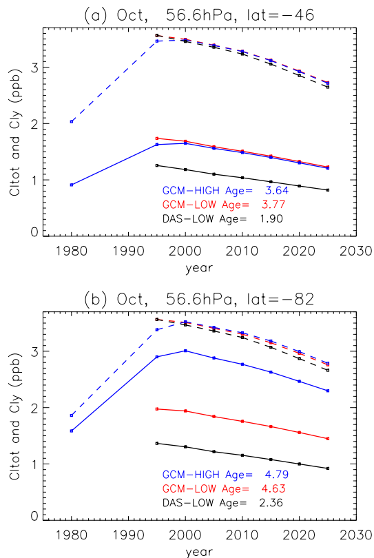
Fig. 3. Time series of October-mean \text{Cl}_y (solid) and \text{Cl}_{\text{tot}} (dashed) for (a) mid-latitude ( 46^\circ \text{S} ) and (b) polar ( 82^\circ \text{S} ) regions.
