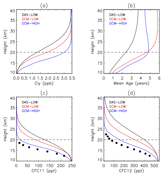
Fig. 2. Vertical profiles of (a) \text{Cl}_y , (b) mean age, (c) CFC11, and (d) CFC12 at 82S. Profiles for \text{Cl}_y are mean values for October 2000, mean age are annual mean values, and CFCs are for September 2005. The solid circles show ACE observations.
