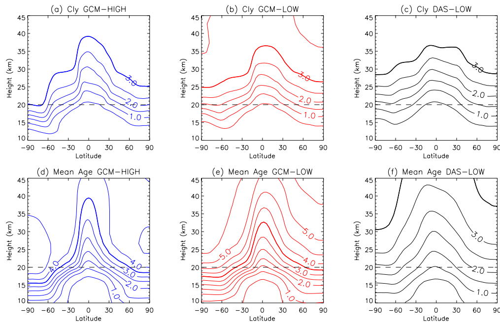
Fig. 1. Contour plots of (a–c; top panels) October-mean \text{Cl}_y , and (d–f; lower panels) annual-mean mean age for 2000, from three CTM simulations. In (a–c) the contour interval is 0.5 ppb, with the 3.0 ppb contour bold, while in (d–e) the contour interval is 0.5 years with 3.5 yr contour bold.
