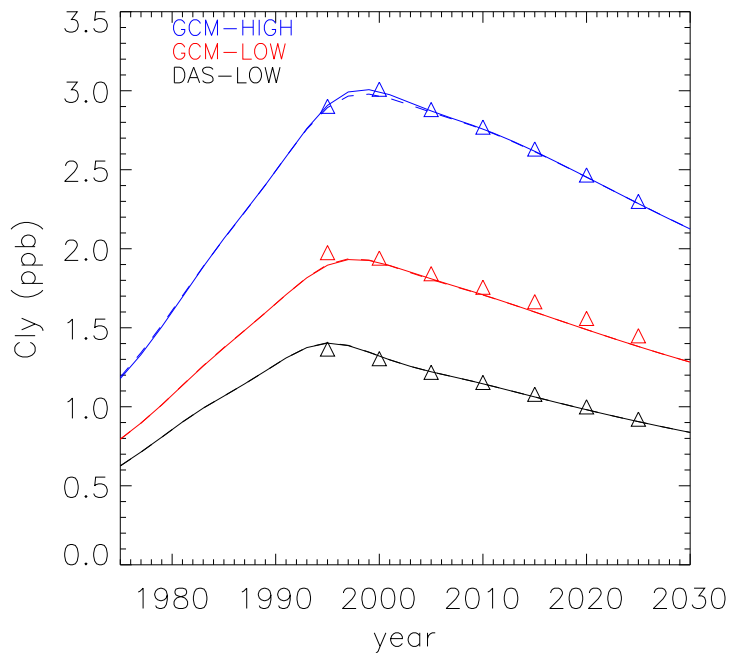
Fig. 4. Comparison of directly simulated \text{Cl}_y at 56.6 hPa and 82° S (symbols) and reconstruction using Newman et al. method (curves), for the three simulations.
