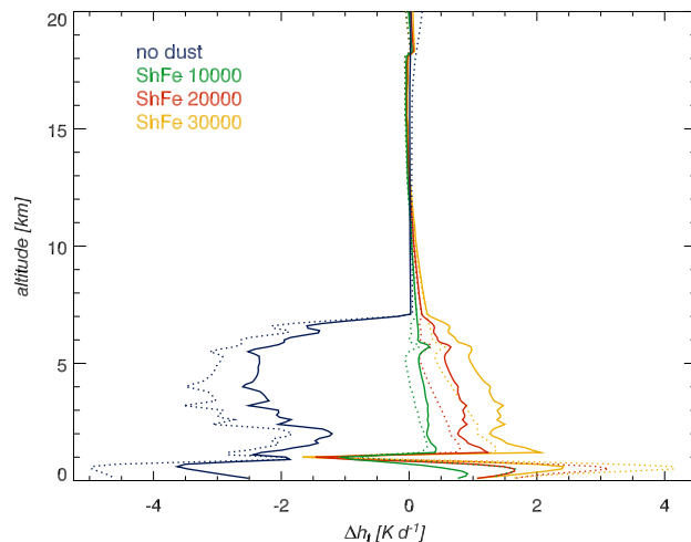
Fig. 10. Profiles of the deviation from the total radiative heating rates of the reference cases ocean (solid) as well as desert (dotted), \Delta h_i(z) , if the measured dust is neglected completely (no dust) or a standard tropospheric aerosol of Shettle and Fenn (1979) is added with surface number concentrations 10 000, 20 000 and 30 000 \text{cm}^{-3} (ShFe10000/20000/30000).
