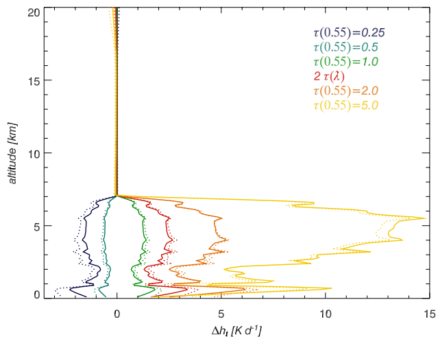
Fig. 11. Profiles of the deviation from the total radiative heating rates of the reference cases of ocean (solid) as well as desert (dotted), \Delta h_t(z) , as function of the scaled measured dust optical depth.
