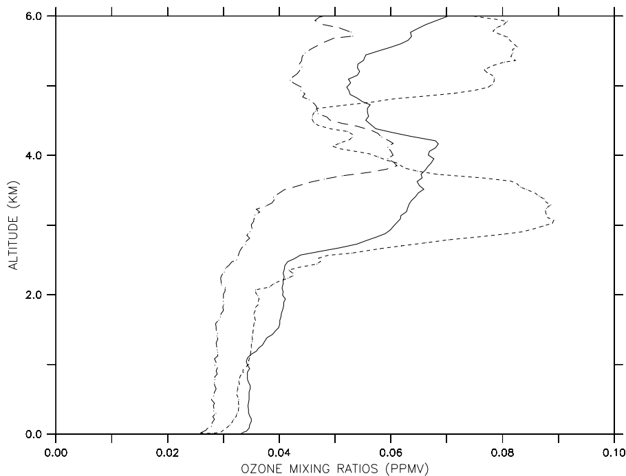
Fig. 5. Ozone mixing ratios measured at Cotonou (6.21° N, 2.23° E) in ppmv on 25 July (solid line), 3 August (dotted line) and 17 August (dashed line).
