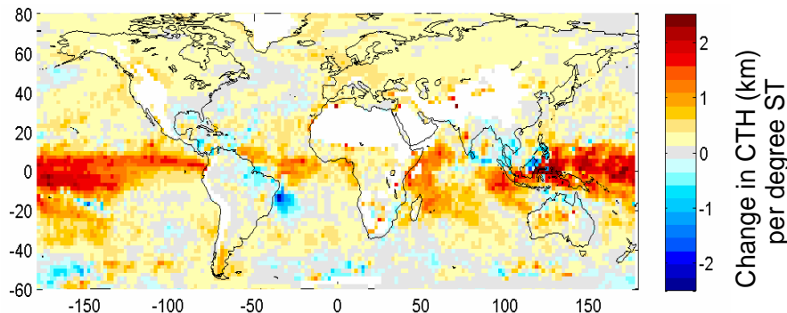
Fig. 8. Absolute changes of the effective cloud fraction (CF, top) and effective cloud top height (CTH, bottom) with increasing surface-near temperature (ST). The changes of the CF are expressed as % (absolute CF) per degree ST; those of the CTH are expressed as km per degree ST. Note that for high latitudes (poleward of about 60^\circ ) our results have increased uncertainties because of the high solar zenith angles and possible interference with ice and snow covered surfaces (see text).
