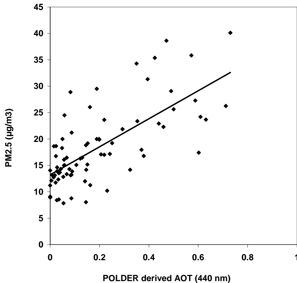
Fig. 4. Comparison between collocated daily averaged PM 2.5 and POLDER derived AOT at 440 nm for a station close to the city of Lille from April to October 2003 ( PM_{2.5}=26.56 AOT_{POLDER}+13.20 , R=0.70 , N=78 , RMS=5.28 ).
