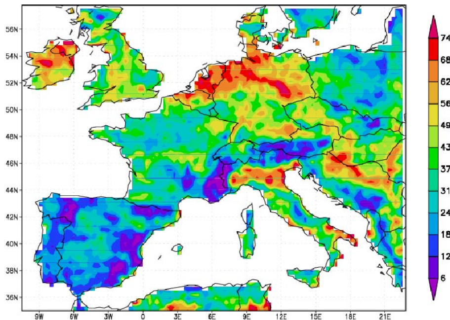
Fig. 6. Number of daily observations with a POLDER AOT above 0.17 and given as a percentage of the total number of observations during the POLDER-2 period (April–October 2003).
