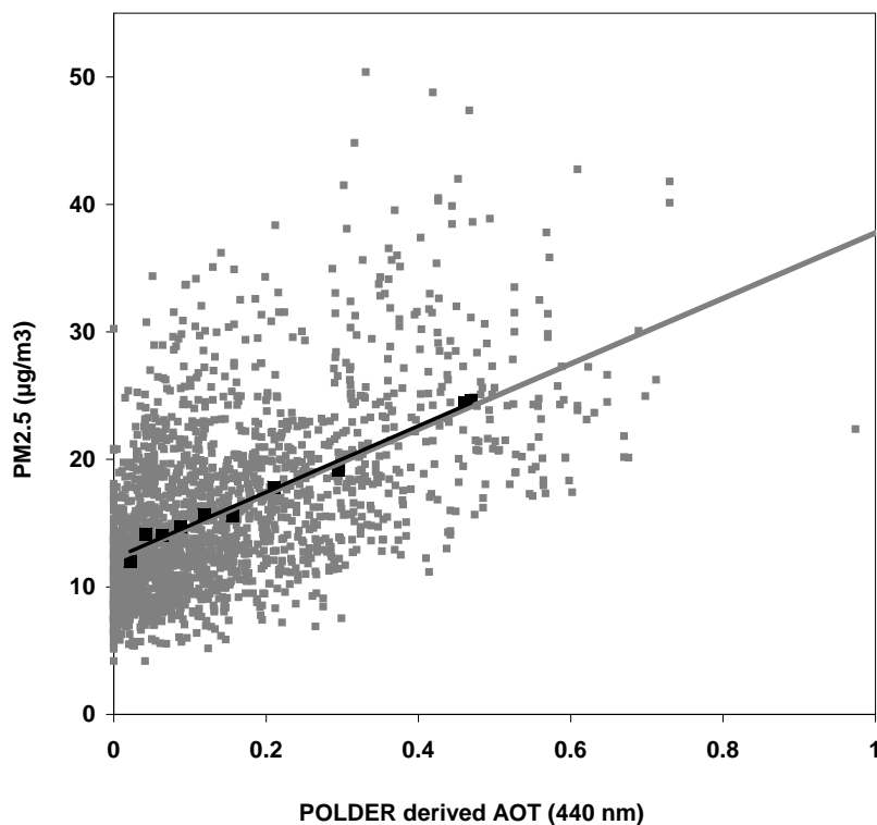
Fig. 5. Regression line between daily POLDER derived AOT at 440 nm and PM 2.5 measured at the ground (Grey dots, PM_{2.5} = 25.67 AOT_{POLDER} + 12.10 , R=0.55 , N=1974 , RMS=5.53 ) over 28 PM stations in France from April to October 2003 and considering the mean values of each of the 10 bins (Black squares, PM_{2.5} = 26.57 AOT_{POLDER} + 12.21 , R=0.99 , N=10 , RMS=0.57 ).
