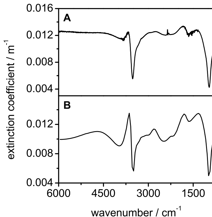
Fig. 7. Panel (A) : Measured infrared extinction spectrum of ice crystals generated by deposition nucleation on mineral dust particles at 237 K. The median size of the ice particles was approximately 13\ \mu\text{m} and their number concentration 30\ \text{cm}^{-3} . Panel (B) : Calculated infrared extinction coefficients of log-normally distributed cylindrical ice particles of aspect ratio \phi=1.0 with the following size distribution parameters: N=30\ \text{cm}^{-3} , \sigma_g=1.15 , and D=13\ \mu\text{m} .
