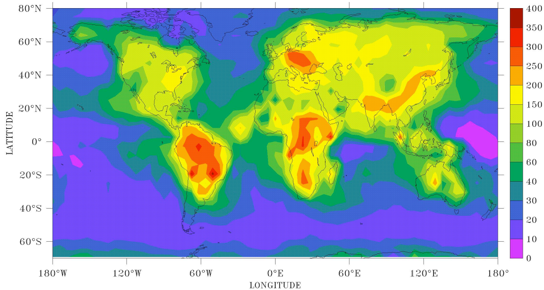
Fig. 1. Global distribution of annually averaged CDNC ( \text{cm}^{-3} ). CDNC is sampled as from a satellite, using the highest cloudy grid box below 500 hPa from each model column.
