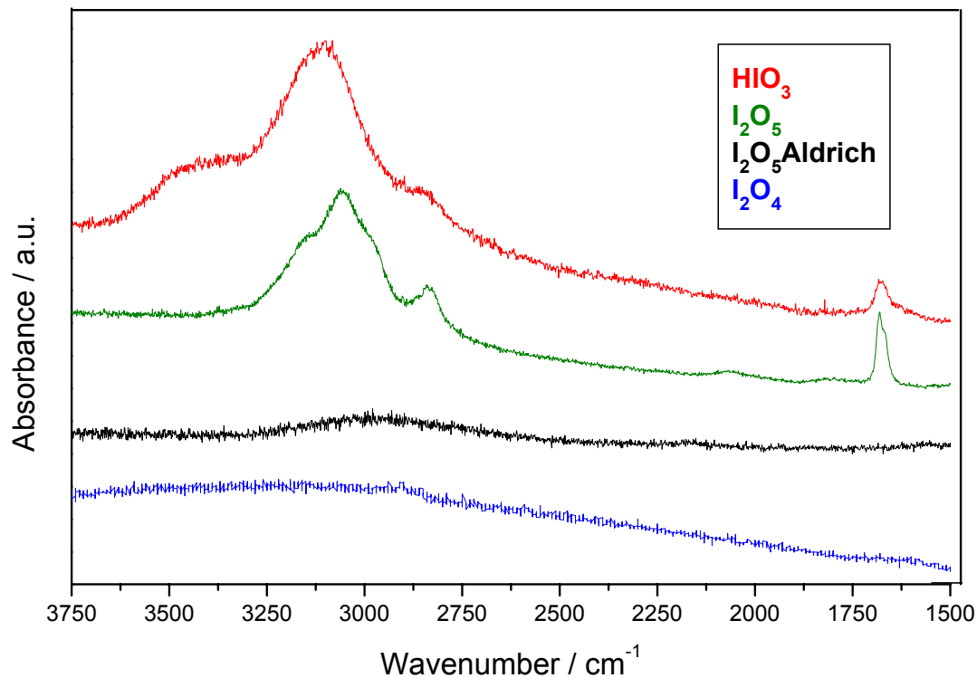
Fig. 6. Raman spectra of HIO 3 , I 2 O 5 and the photochemically produced aerosols together with I 2 O 5 powder (from Aldrich) in the range 4000–1000 cm -1 .
