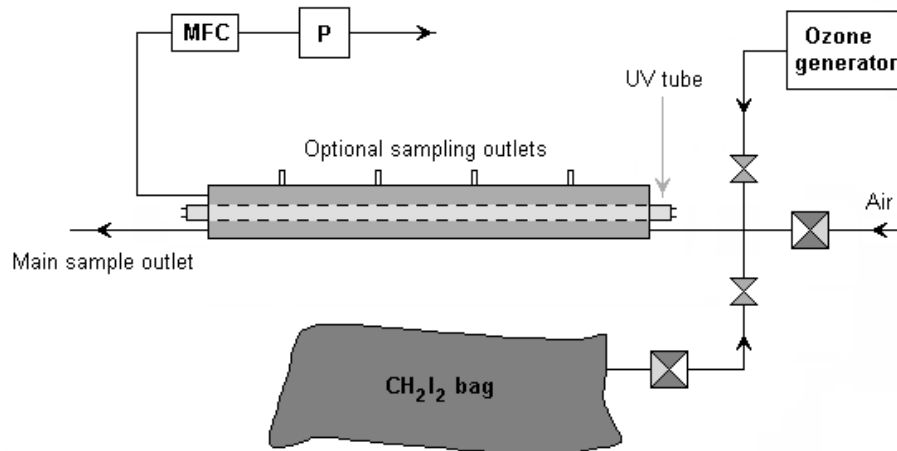
Fig. 2. Photochemical reactor set-up. The chamber has optional outlets along the side to allow determination of the progress in aerosol growth. MFC – mass flow controller; P – pump.
