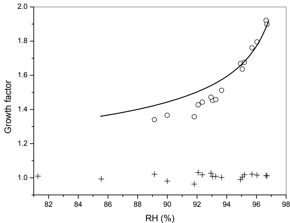
Fig. 8. Hygroscopic growth factor versus relative humidity for 90 nm \text{HIO}_3 particles heated to 220^\circ\text{C} in a sheath of \text{N}_2 : circles – hygroscopic growth factor, crosses – non-hygroscopic growth factor, full line – model predictions for \text{HIO}_3 particles.
