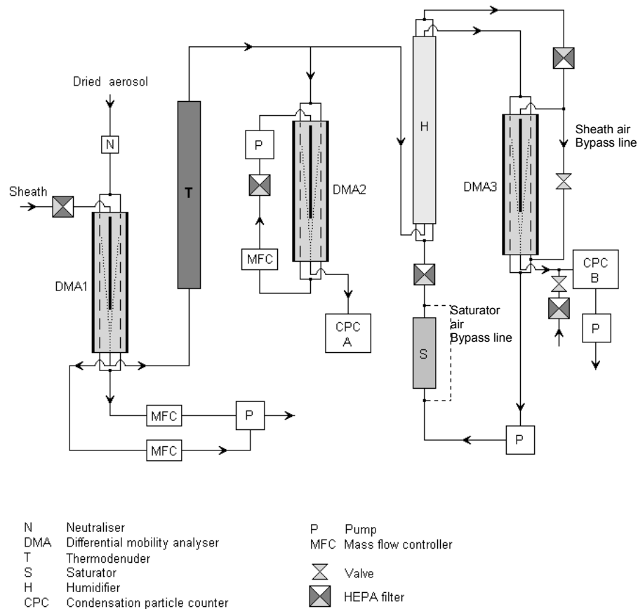
Fig. 1. Schematic diagram of the VH-TDMA system.
