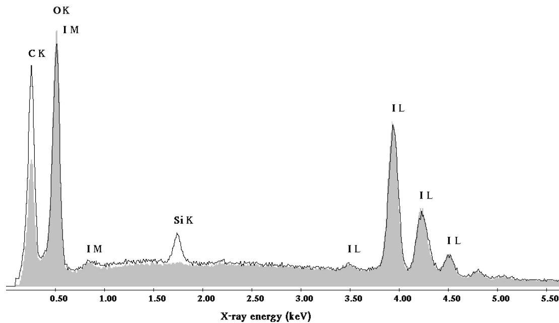
Fig. 7. I_2O_5 (in light grey) and the photooxidation product (black line) comparison spectra.
