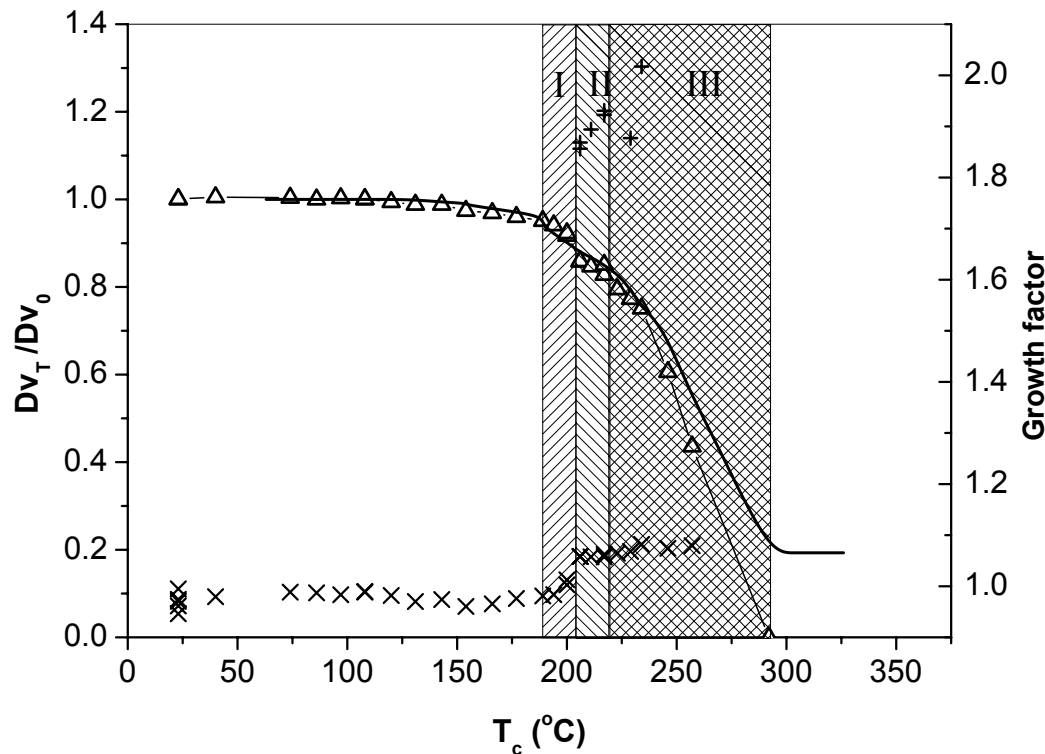
Fig. 4. VH-TDMA spectra of 80 nm photochemically produced aerosols, showing the relative diameter after volatilisation Dv_T/Dv_0 – triangles; and the hygroscopic growth factors G=D_h/D_v versus thermodenuder temperature, for both hygroscopic G_h (+) and non-hygroscopic G_{nh} (x) peaks. The sheath gas was filtered air. The volatility curve of HIO_3 particles of similar size measured in air as sheath gas is also shown with a full line.
