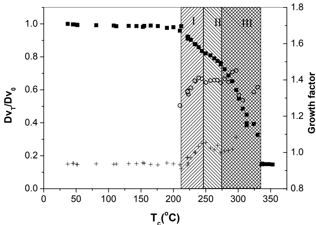
Fig. 3. VH-TDMA spectra of HIO 3 particles with an initial diameter of 75 nm, showing the relative diameter after volatilisation Dv_T/Dv_0 – full squares; and the hygroscopic growth factors G=D_h/D_v versus thermodenuder temperature, for both hygroscopic G_h (circles) and non-hygroscopic G_{nh} (crosses) peaks. Nitrogen was used as the sheath gas.
