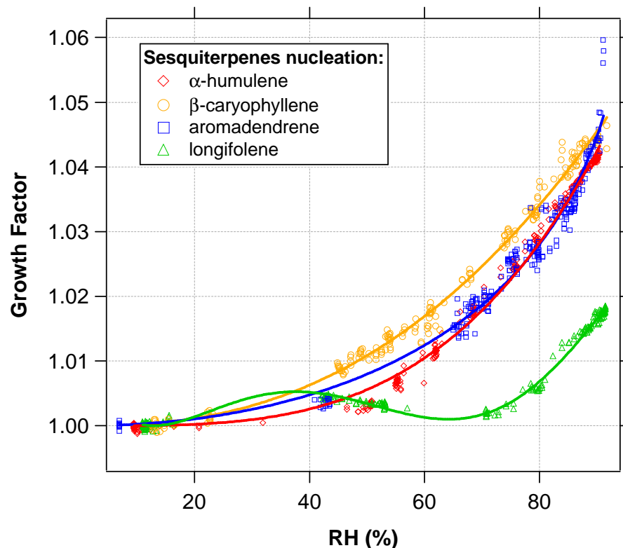
Fig. 10. Hygroscopic growth curves for nucleated SOA formed by sesquiterpene photooxidation. Sesquiterpene SOA exhibits very low hygroscopicity, showing smooth but very small water uptake, with growth factors mostly between 1.01–1.04 at 85% RH. While the shapes of the curves for SOA from \alpha -humulene, \beta -caryophyllene, and aromadendrene are similar, the curve for longifolene exhibits an unexpected behavior, in which the increase in GF with RH is not monotonic. This could be indicative of the presence of void volumes in the particle, which can lead to compaction of the structure after a certain degree of water uptake.
