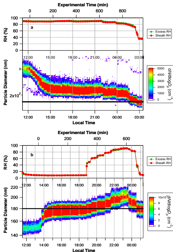
Fig. 2. Image plots of raw TDMA data and the variations in RH in a typical operating scheme for (a) cycloalkene ozonolysis experiments (dry) and (b) terpene photooxidation experiments (humid). The data shown here are from ozonolysis of 181 ppb of methylene cyclohexane in the presence of (\text{NH}_4)_2\text{SO}_4 seed and photooxidation of 105 ppb verbenone in the presence of (\text{NH}_4)_2\text{SO}_4 seed, respectively. The thick black line in each image plot denotes the classified particle size of 180 nm.
