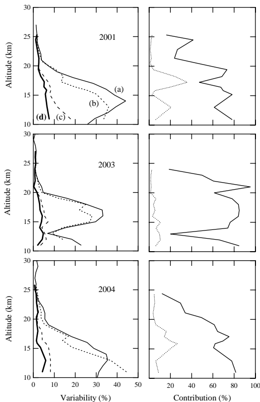
Fig. 3. Analysis of contributions to zonal variability (relative standard deviation) of ozone in 2001 (top), 2003 (middle) and 2004 (bottom). Left: percent variability (a) number density at constant altitude (b) mixing ratio on isentropic surfaces; (c) after removing horizontal transport; (d) after removing vertical and horizontal transport. Right: relative contributions of horizontal (solid line) and vertical (dotted) transport to total variability.
