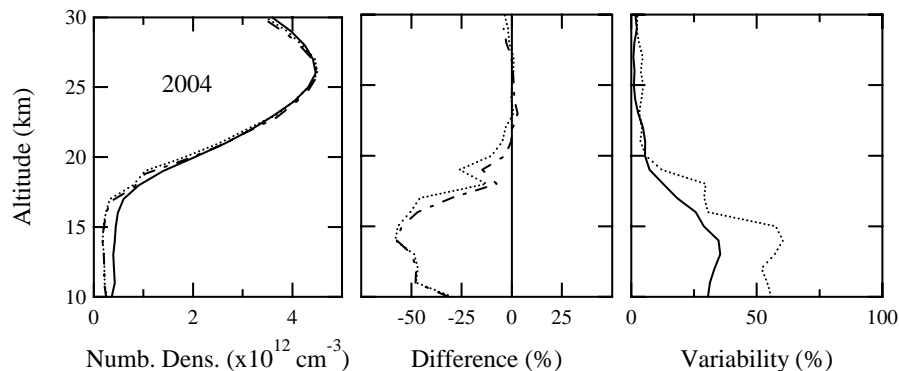
Fig. 4. Comparison between SAOZ and SHADOZ ozonesondes in 2004. From left to right: mean zonal profile, relative percent difference compared to the mean and relative standard deviation. Solid line: SAOZ; dotted: SHADOZ; dotted-dashed: SHADOZ altitude adjusted for bias.
