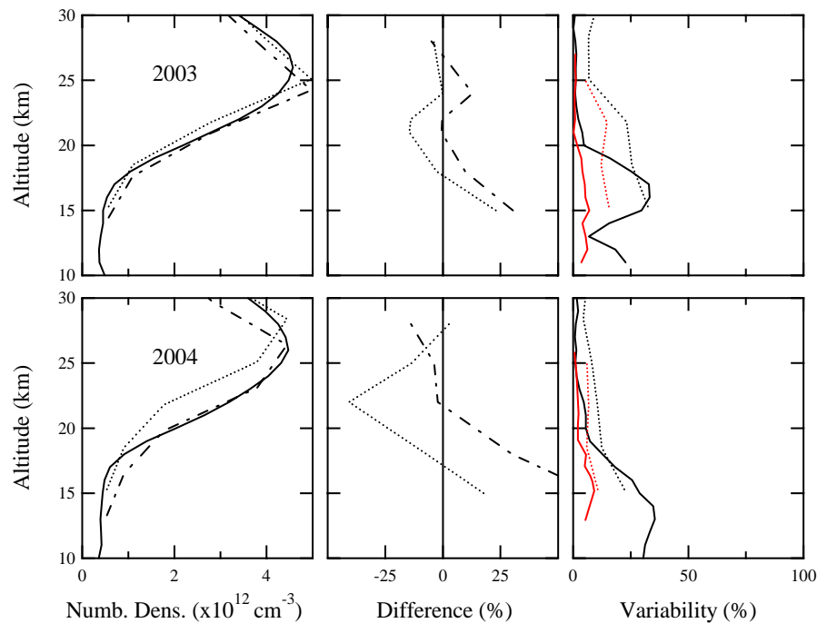
Fig. 12. Same as Fig. 6 but for SCIAMACHY (dotted), altitude adjusted (dotted-dashed) and SAOZ (solid).
