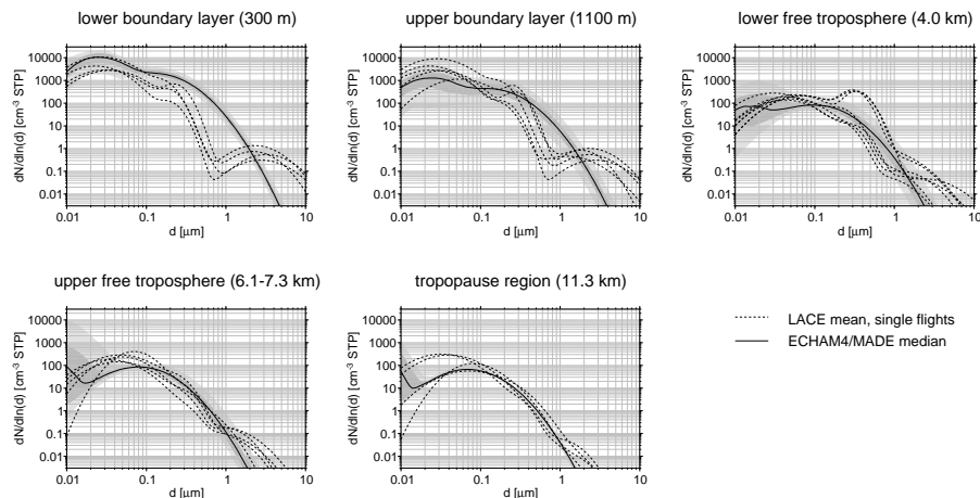
Fig. 13. Number size distributions at different altitudes obtained from averaged measurements during the LACE campaign over northeastern Germany (dashed) (Petzold et al., 2002) and the corresponding median size distribution calculated by ECHAM4/MADE (solid). The shaded areas indicate the 25%- and 75%- resp. 5%- and 95%-percentiles of the model results.
