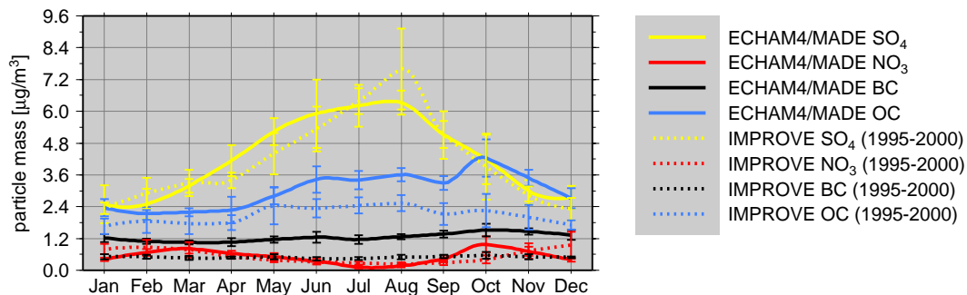
Fig. 5. Climatological seasonal cycle of observed and modeled mass concentrations of the aerosol components \text{SO}_4 , \text{NO}_3 , BC, and OC in fine particles ( \text{PM}_{2.5} ), averaged over the south-eastern part of the USA. The error bars denote the standard deviation of the individual monthly means to the climatological average.
