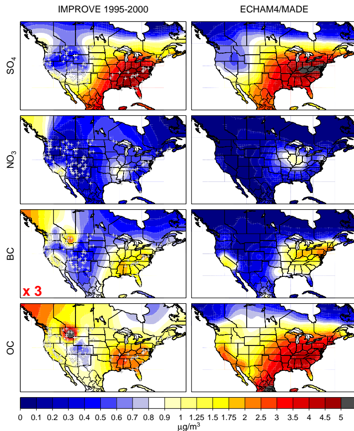
Fig. 6. Climatological annual means of the mass concentrations of SO 4 , NO 3 , BC, and OC in fine particles (PM 2.5 ) obtained from measurements of the IMPROVE network (left) and from model results of ECHAM4/MADE (right). The measured BC concentrations have been multiplied by 3 (“x 3”). The white crosses denote the locations of the measurement sites.
