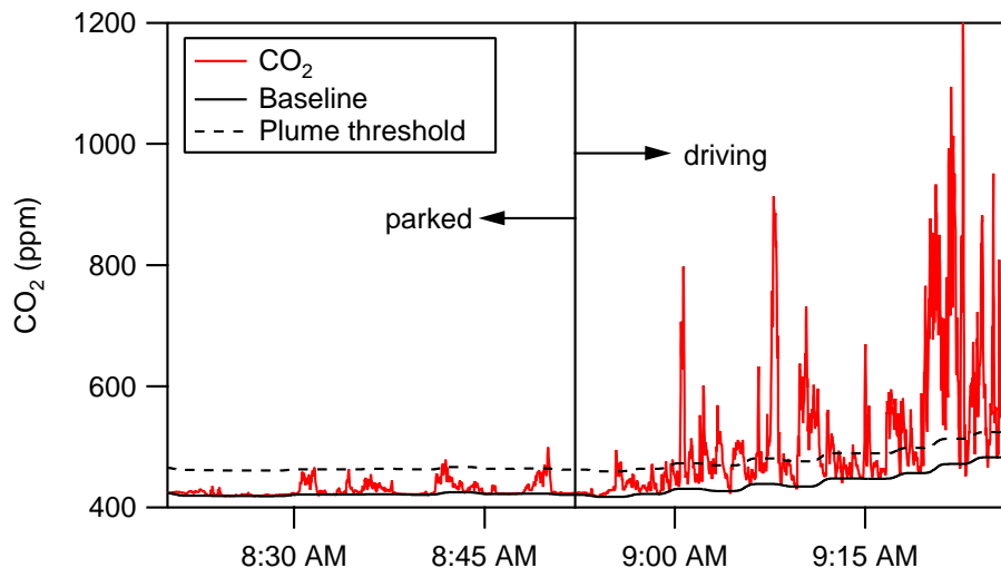
Fig. 2. CO 2 concentrations measured by the mobile lab on 1 May 2003. The van was parked at the supersite until 8:52 a.m., at which time it began driving. Data points above the plume threshold (42 ppm above baseline) during the driving period are considered potential exhaust plumes.
