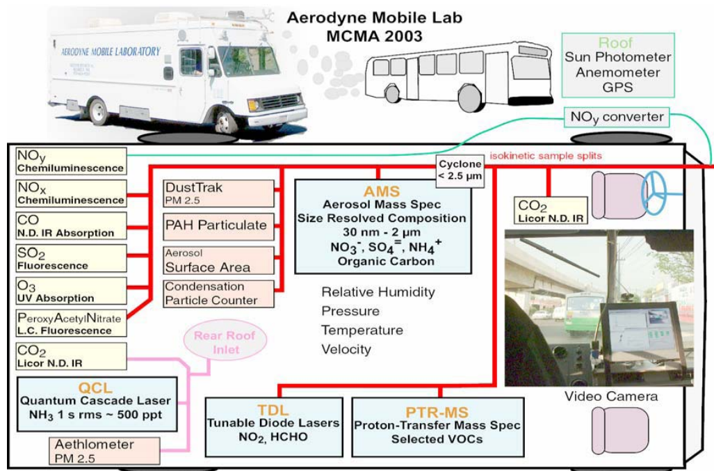
Fig. 1. Schematic of the Aerodyne mobile lab as instrumented for the MCMA-2003 field campaign.
