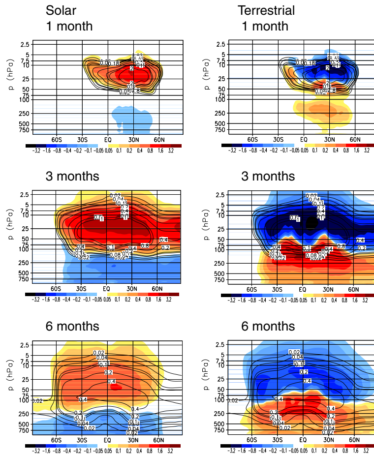
Fig. 4. Anomalies of the monthly mean zonally averaged solar (left panel) and terrestrial (right panel) heating rates (K/day) caused by a Yellowstone super eruption in YESTJUN for different months after the eruption. The contour lines indicate the aerosol mass mixing ratio (ppm S).
