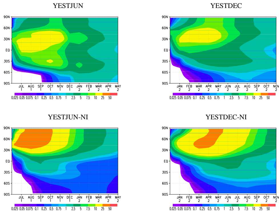
Fig. 2. Optical depth at 0.5 \mu\text{m} for the four experiments. Numbers at the abscissae indicate month and year after the eruption.
