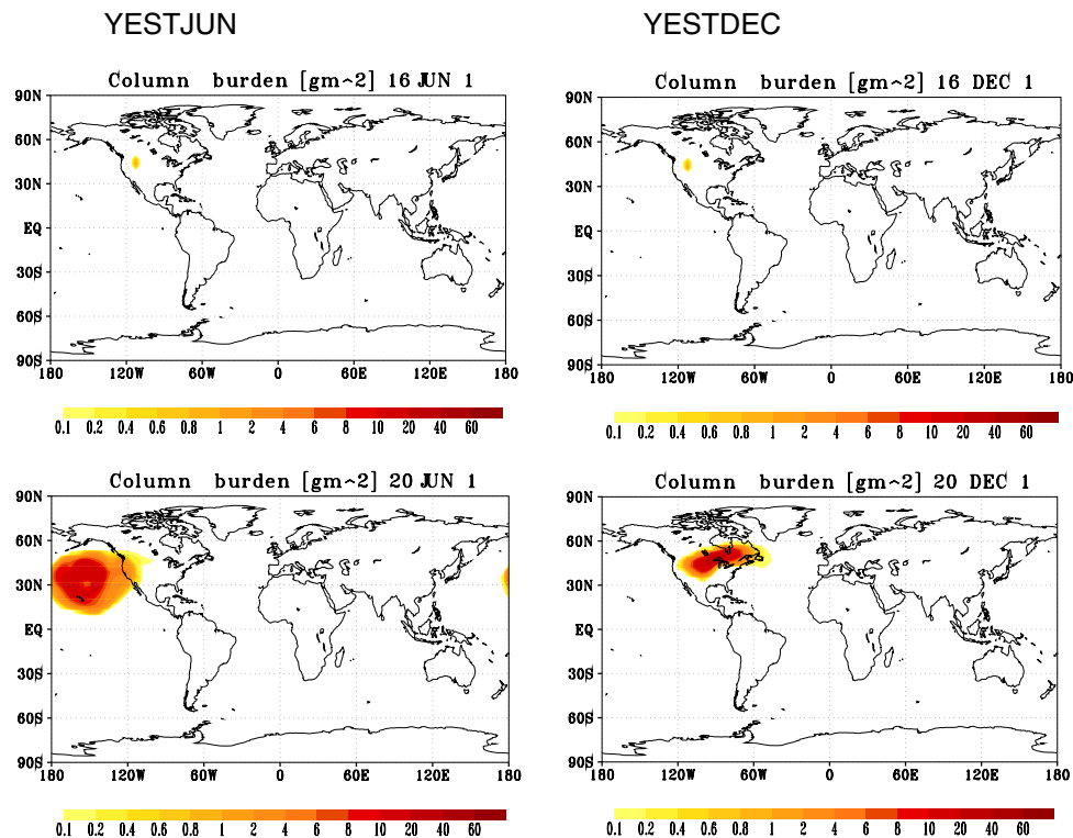
Fig. 1. Geographical distribution of aerosol column burden in both experiments for the first month after the eruption.
