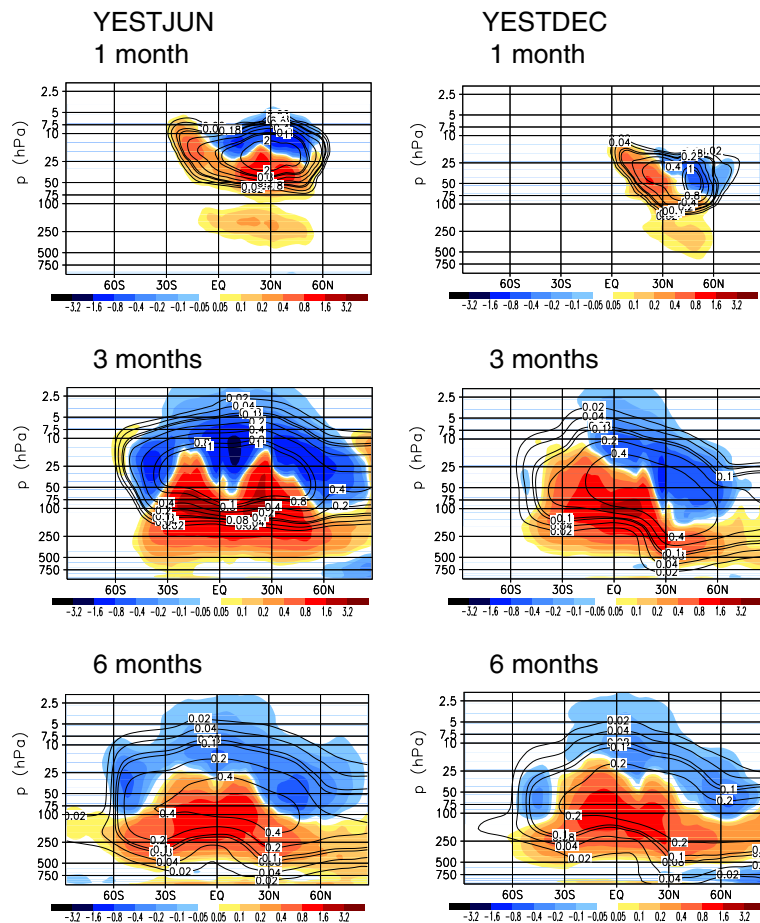
Fig. 3. Anomalies of the monthly mean zonally averaged total heating rates (K/day) caused by a Yellowstone super eruption in both experiments for different months after the eruption. The contour lines indicate the aerosol mass mixing ratio (ppm S).
