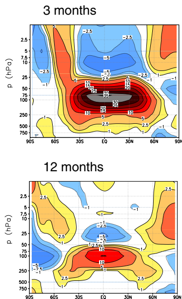
Fig. 7. Monthly and zonal mean temperature difference between the interactive (including aerosol effects) and the noninteractive simulation (excluding aerosol effects) for YESTJUN.
