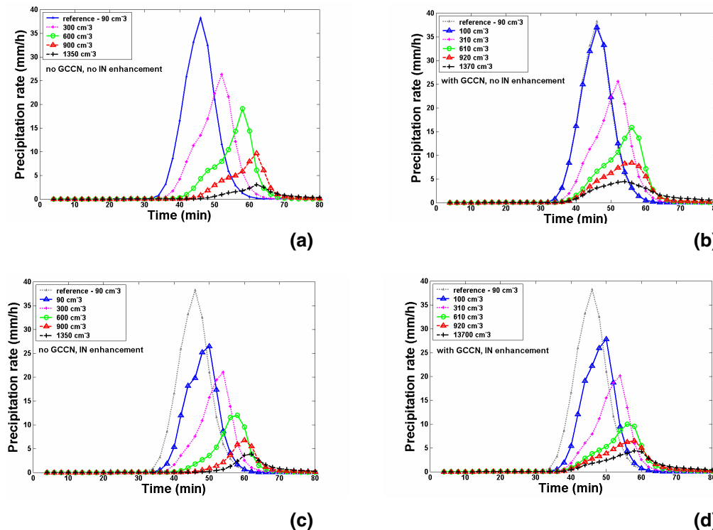
Fig. 4. Precipitation rate as function of time for the entire cases. (a) corresponds to cases in which GCCN are not present and IN concentration is not enhanced, (b) corresponds to cases in which GCCN are added and IN concentration is not enhanced, (c) corresponds to cases in which GCCN are not present and IN concentration is enhanced, (d) corresponds to cases in which GCCN added and IN concentration is enhanced.
