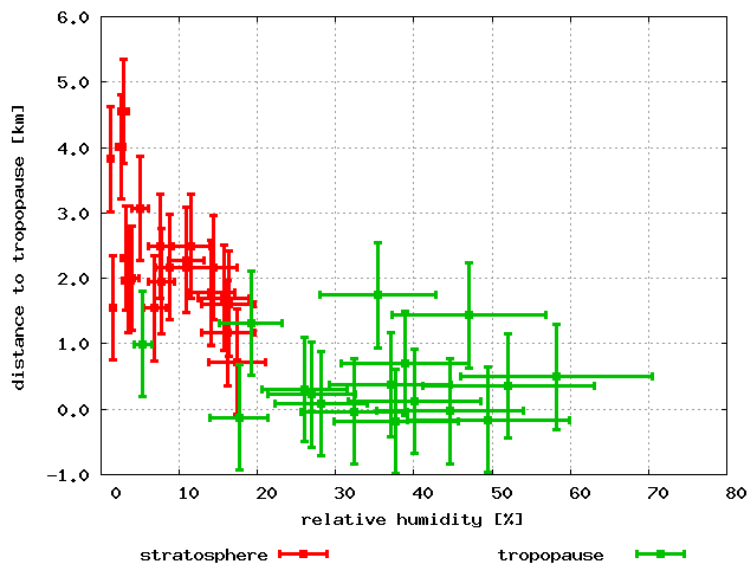
Fig. 3. Relative Humidity plotted versus distance to the tropopause. As the relative humidity is below saturation and decreases with distance above the tropopause, the decrease in water vapor mixing ratio cannot be a continuous condensation process but must be due to mixing of moist air from tropopause level with dry stratospheric air.
