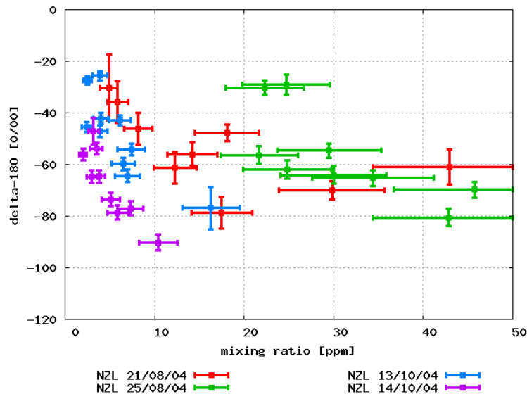
Fig. 4. \delta^{18}\text{O} plotted versus mixing ratio. The tropopause samples with \nu > 10 ppm show no correlation between mixing ratio and \delta^{18}\text{O} , whereas the individual stratospheric datasets appear to share a common slope (see Fig. 5).
