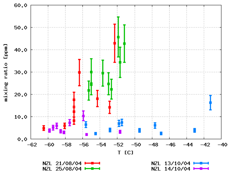
Fig. 1. H 2 O mixing ratio plotted versus ambient temperature. The samples can clearly be separated into stratospheric samples with \nu < 10 ppm, and samples from the tropopause region, which show a correlation between H 2 O mixing ratio and temperature. The legend gives the flight dates.
