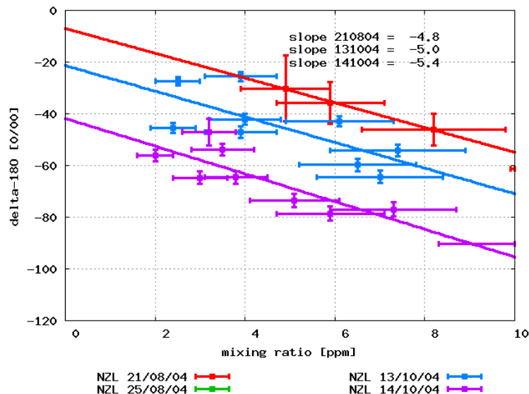
Fig. 5. \delta^{18}\text{O} of the stratospheric samples plotted versus mixing ratio. \delta^{18}\text{O} increases with decreasing mixing ratio in the stratosphere; the individual datasets share the same slope.
