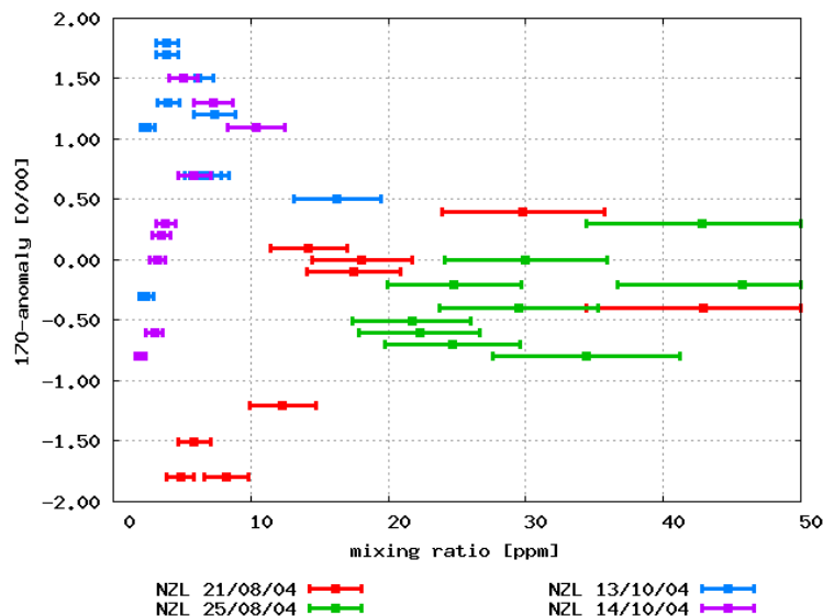
Fig. 7. \Delta^{17}\text{O} plotted versus water vapor mixing ratio. No significant oxygen isotope anomaly can be deduced from the data. The error of \Delta^{17}\text{O} is \sim 0.35 for the larger samples with \nu \sim 50 ppm, and increases with lower mixing ratios.
