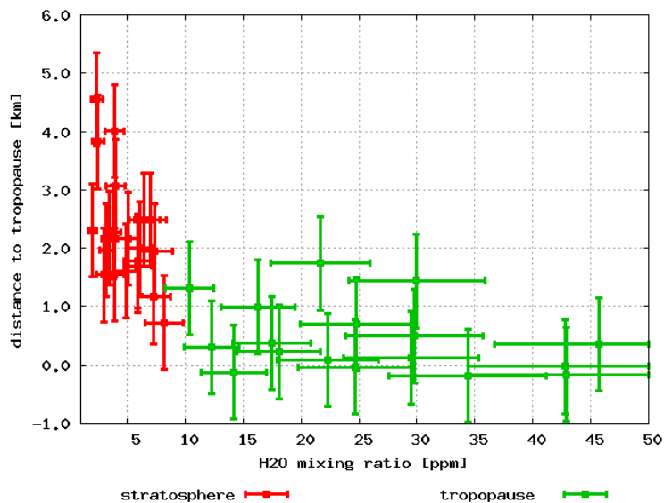
Fig. 2. H 2 O-mixing ratio plotted versus distance to the tropopause. A decrease in mixing ratio with increasing distance to the tropopause is visible for the stratospheric samples, which is due to mixing of relatively moist air from the tropopause cold point with dry stratospheric air from above.
