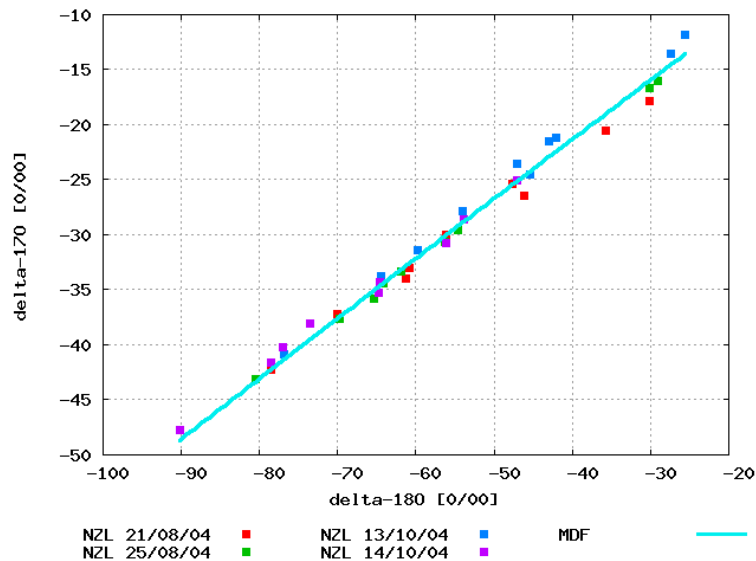
Fig. 6. Three-isotope plot of \delta^{17}\text{O} versus \delta^{18}\text{O} . Also shown is the terrestrial mass-dependent fractionation line, defined as \Delta^{17}\text{O}=0 (see Eq. 2). The data points scatter symmetrically around the mass-dependent fractionation line, and the deviations are further examined in Fig. 7.
