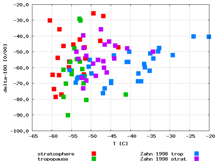
Fig. 8. Comparison of the \delta^{18}\text{O} data with measurements by Zahn et al. (1998) in a plot versus temperature. The correlation with temperature is pronounced in the samples of Zahn et al. (1998) because most of their samples were taken at or below the tropopause. Above the tropopause, the data from Zahn et al. (1998) show the same behavior as the data presented here: high variability and a trend towards higher \delta values.
