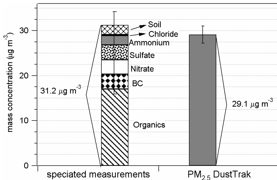
Fig. 10. Estimation of the total PM 2.5 mass concentration from AMS, BC, and soil mass concentration, compared with PM 2.5 DustTrak mass concentration. Averages were carried out over all time intervals for which all data (AMS, BC, soil, and DustTrak) were available.
