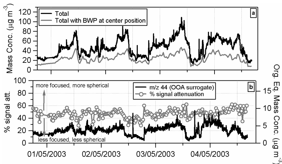
Fig. 5. Panel (a): time series of the AMS Total mass concentration (when the beam width probe (BWP) was in the “out position”), and the mass concentration measured when the BWP was blocking the particle beam at the center position. Panel (b): signal attenuation caused by the BWP at the center position, and time series of the AMS fragment m/z 44 (marker for oxygenated organics (OOA)) in Org. Eq. Mass Concentration. The mass concentrations in this graph were not corrected for air beam variations.
