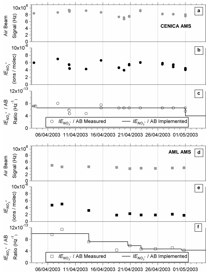
Fig. 1. Summary of the results of the ionization efficiency calibrations of the CENICA (panels a–c) and Mobile Laboratory (panels d–f) AMSs during the MCMA-2003 field campaign.
