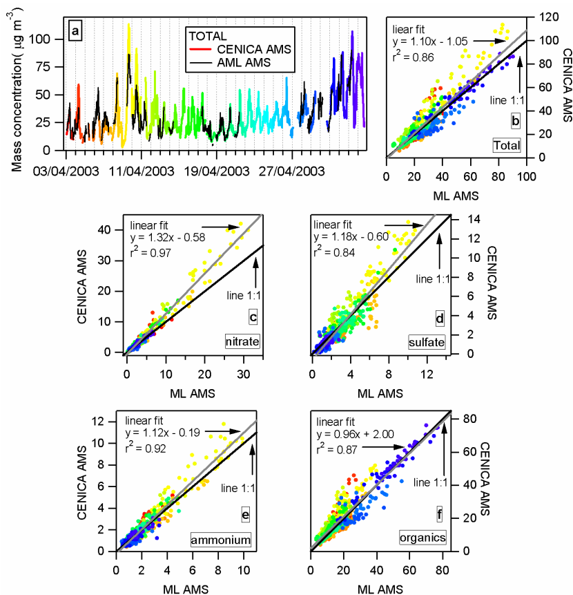
Fig. 6. Panel (a): comparison of the time series of Total NR-PM 1 measured with the CENICA and the mobile laboratory AMSs, for periods when the AML was parked at CENICA during MCMA-2003. Panels (b) through (f): scatter plots of the Total NR-PM 1 , and its species, measured with the CENICA and the mobile laboratory AMSs. Black lines are 1:1 lines. Grey lines are linear fits to the data. The data is presented in 30 min averages.
