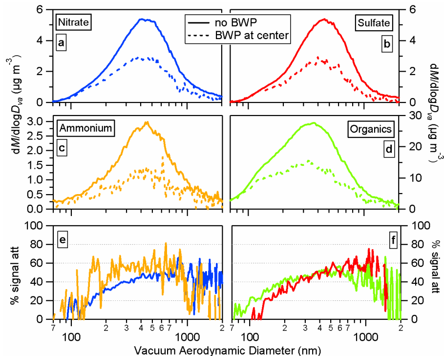
Fig. 4. Panels (a) through (d): Campaign-average size distributions obtained by the CENICA AMS without the BWP and with the BWP blocking the particle beam at the center position. Panels (e) and (f): signal attenuation caused by the BWP at the center position as a function of particle size.
