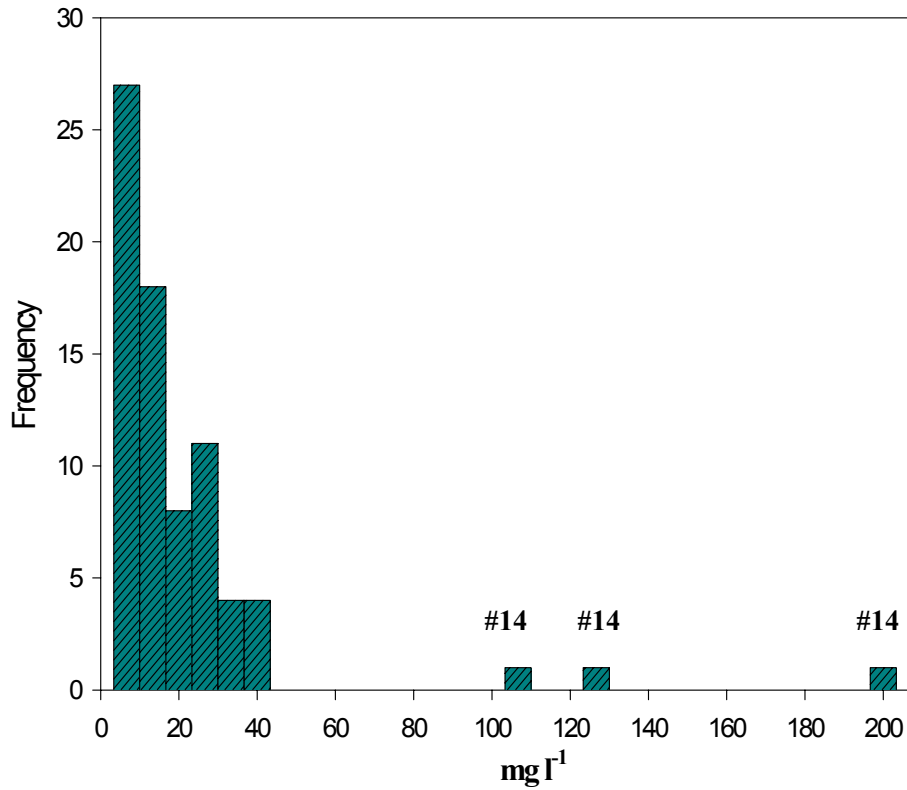
Fig. 1. Frequency distribution of Total Ionic Content in cloud water samples.
