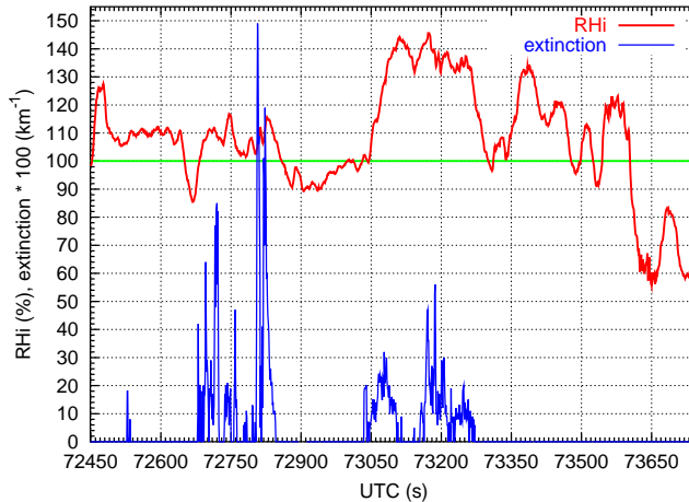
Fig. 11. Time series measurements of RHi (in %, red curve) and extinction (in \text{km}^{-1} , scaled by 100, blue curve) along a research flight of 3 April 2000 during the INCA campaign over Punta Arenas, Chile (see e.g. Ovarlez, 2002; Gayet, 1997). Ice saturation is marked by the green line. The time resolution of the data is one second. The data show how cirrus clouds are embedded in the ISSR that extends over almost the whole flight segment (pressure \approx 286 hPa). Note also the clear but supersaturated portions.
