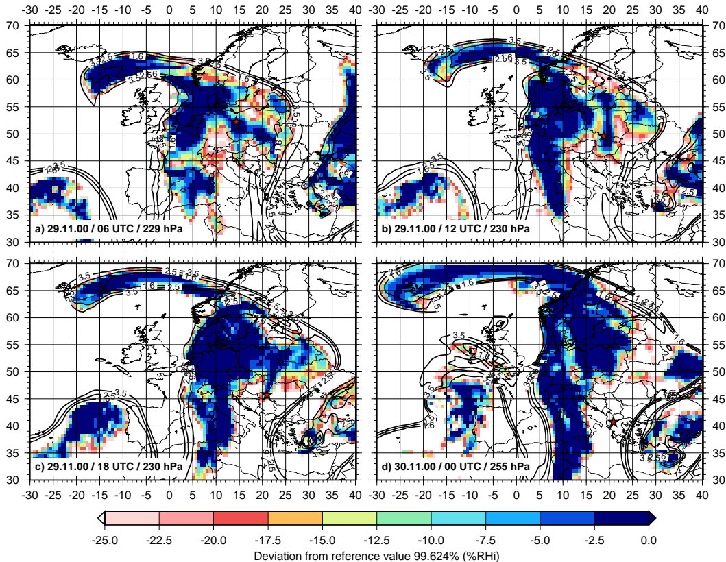
Fig. 9. Evolution of the ice supersaturation layer, measured by the radiosonde at 29 November 2000, 06:00 UTC along the trajectory Tr_{31,1} —part 2: (a) t=\pm 0 h, p=229 hPa; (b) t=+6 h, p=230 hPa; (c) t=+12 h, p=230 hPa; (d) t=+18 h, p=255 hPa. The reference value of RH_i has been taken from the comparison of the radiosonde and ECMWF data at t=\pm 0 (radiosonde ascent). The position of the trajectory is marked by a red star. The solid black lines are as in Fig. 8.
