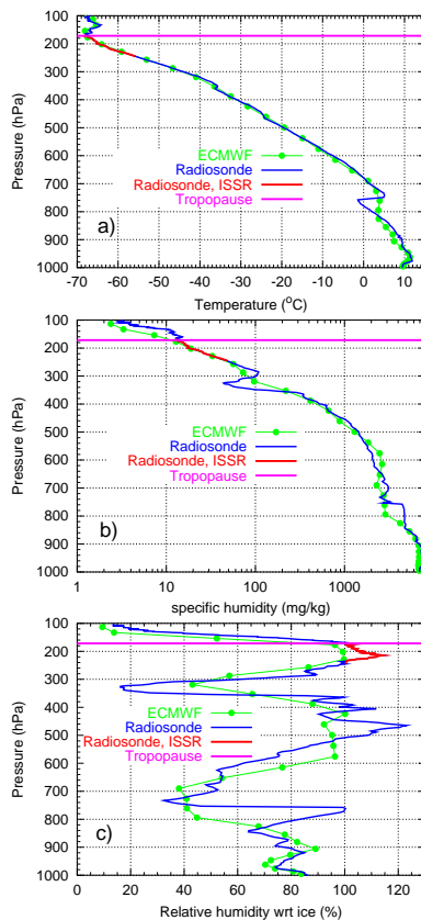
Fig. 3. Vertical profiles of the radiosonde (blue curve) and the corresponding values from the ECMWF data set (green filled circles and curve, values picked from the nearest grid points at every model level). Additionally, the thermal tropopause (pink line) and the reported ice supersaturated layer (red curve) obtained from the radiosonde are shown. (a) Temperature in degree Celsius; (b) Specific humidity in milligrams water vapour per kilogram dry air; (c) Relative humidity with respect to ice in percent.
