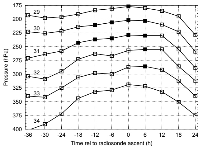
Fig. 7. Formation and evolution of the ISSR (filled square) along the main trajectories Tr_{29,1} - Tr_{34,1} (lines with open squares). The time is shown relative to the radiosonde ascent at 29 November 2000, 06:00 UTC.
