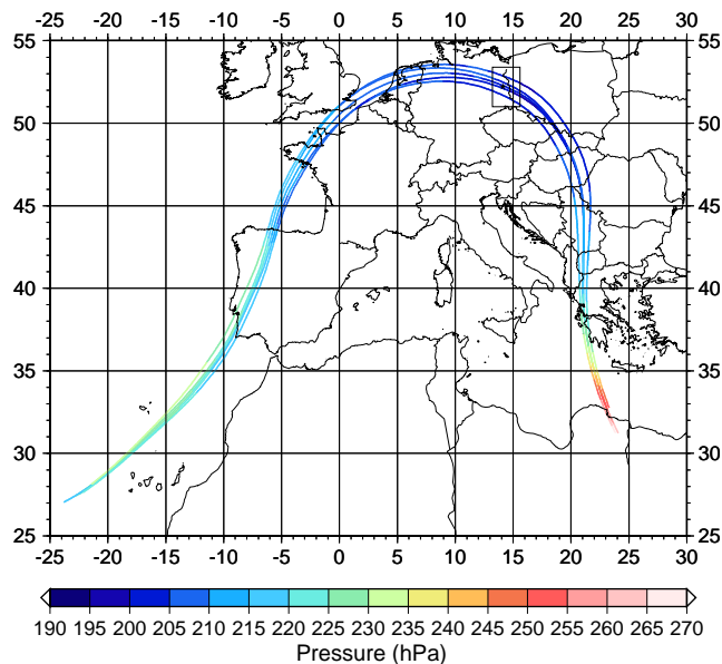
Fig. 5. Trajectories Tr_{30,1} – Tr_{30,5} for the time period from 27 November 2000, 18:00 UTC to 30 November 2000, 06:00 UTC. The vertical coordinate is indicated by the colour bar.
