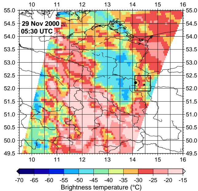
Fig. 4. Infra-red METEOSAT picture of the region “GermanyNE” (9.5–16° E, 49.5–55° N) at 05:30 UTC. Additionally, the positions of Lindenberg and of the air parcels measured by the radiosonde (filled triangle) are shown. Also, the nearest ECMWF grid point (open square, center at 14.4° E/52.2° N, extension 0.6°×0.6°) is shown.
