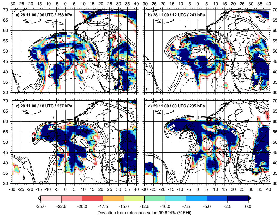
Fig. 8. Evolution of the ice supersaturation layer, measured by the radiosonde at 29 November 2000, 06:00 UTC along the trajectory Tr_{31,1} —part 1: (a) t=-24 h, p=258 hPa; (b) t=-18 h, p=243 hPa; (c) t=-12 h, p=237 hPa; (d) t=-6 h, p=235 hPa. The reference value of RH_i has been taken from the comparison of the radiosonde and ECMWF data at t=\pm 0 (radiosonde ascent). The position of the trajectory is marked by a red star. The solid black curves mark potential vorticities of 1.6, 2.5, and 3.5 PVU, respectively.
