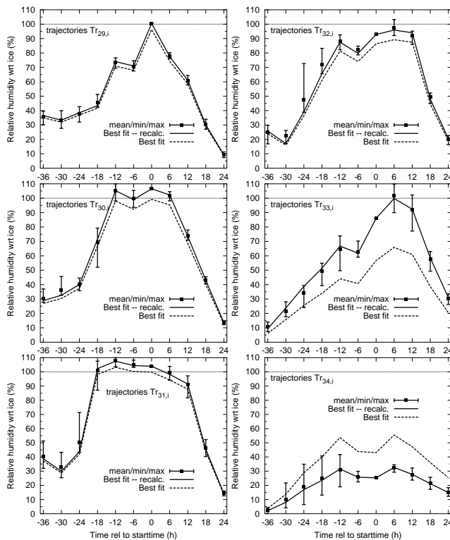
Fig. 6. Relative humidity along the mean trajectories as reported in the ECMWF data set (dashed curves) and recalculated using the tendencies of specific humidity (solid curves). Additionally, the minima, maxima and the mean values of the recalculated RH_i values along the five trajectories (error bar and filled square) are presented.
