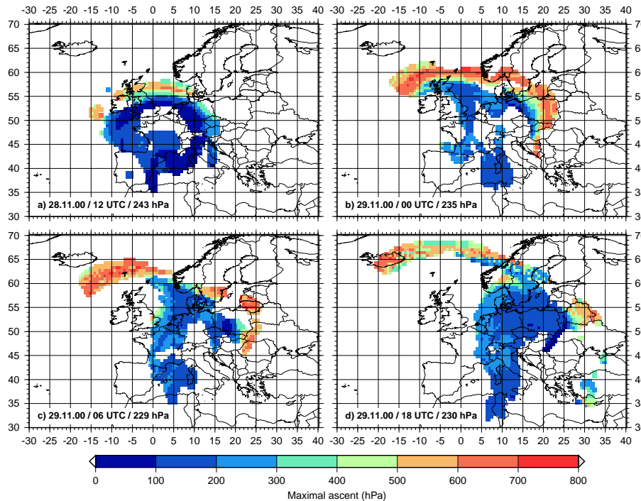
Fig. 10. The maximal ascent of 48 h trajectories (24 h in the upper left panel) are shown for some of the ISSR areas of Figs. 8 and 9: (a) t = -18 h, p = 243 hPa; (b) t = -6 h, p = 235 hPa; (c) t = 0 h, p = 229 hPa; (d) t = +12 h, p = 230 hPa. This makes evident two different categories of ISSRs: The first one, marked in blue is characterised by a weak ascent of all air parcels in the investigated column. The second one, marked in reddish colours, is more directly influenced by the outflow of the warm conveyor belt which results in a very strong ascent for at least one trajectory in the respective column. An intermediate category of maximum ascents (green colours) seems to be unimportant, at least in the situation investigated here.
