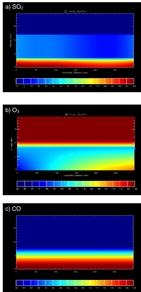
Fig. 3. Initial concentration for chemical compound (a) SO 2 (ppbv), (b) O 3 (ppbv), and (c) CO (ppbv).
