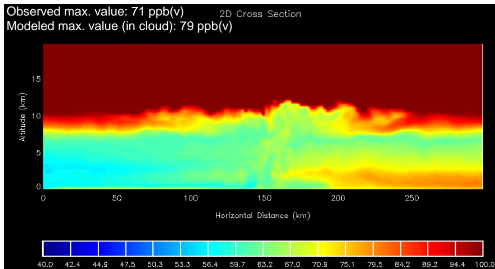
Fig. 5. (i) Modeled O_3 concentration (ppb) after 3 h simulation. Modeled and observed values at 10.4 km are indicated in the figure.
