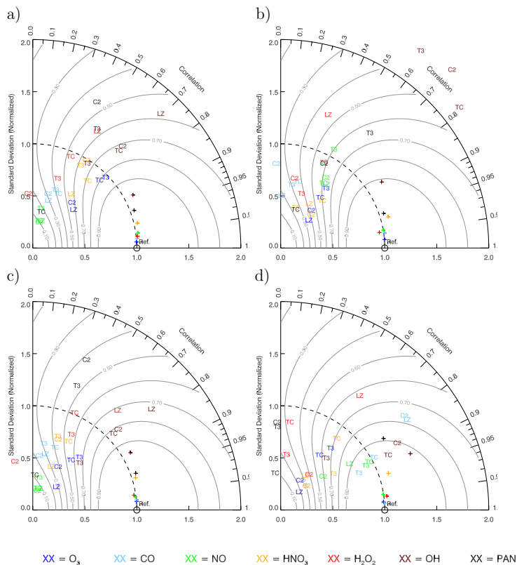
Fig. 7. Taylor diagrams of model performance for the SONEX campaign. (a) All measurements at p < 350 hPa (same data as in 4), (b) early flights 3–7 only, (c) late flights 9–16 only, (d) vertical profiles at Shannon (same data as in Fig. 5). For further explanations refer to 6.
