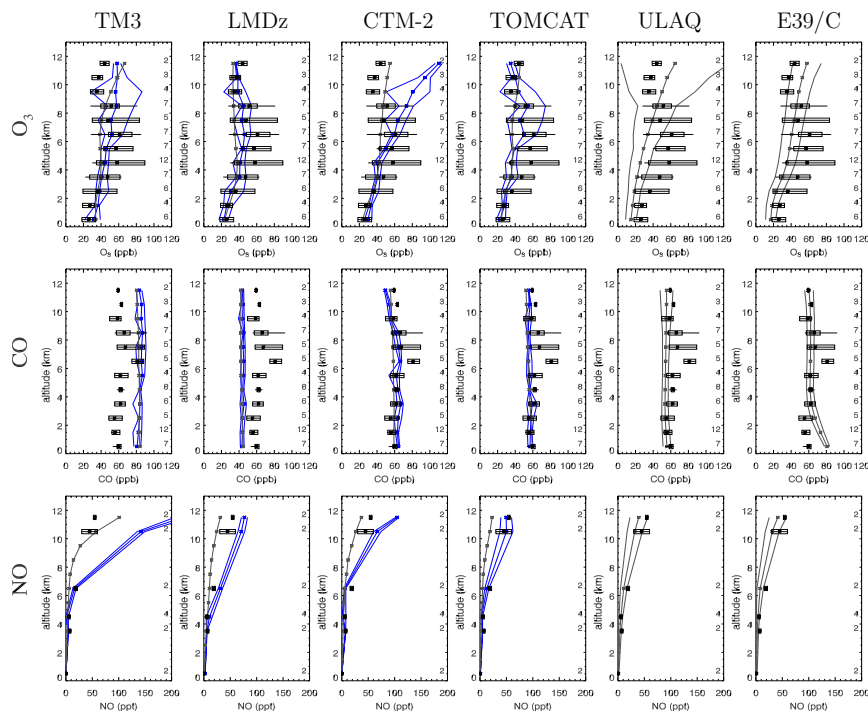
Fig. 3. (a) PEM-Tropics A profiles at at Tahiti, 17.5° S/149.5° W. Horizontal bars and boxes span the central 90% and 67% of the frequency distributions of the measurements grouped into individual 1 km altitude bins. Mean values are indicated by a star inside each box. Blue solid lines represent the corresponding model values. The central thick line connects the model mean values and the range between the two thinner lines represents the central 67% range calculated from the point-by-point model output. The dark grey line shows the monthly mean profile of the model grid column containing Tahiti for September 1996. This profile can be compared to the mean model profile derived from the point-by-point output. For E39/C and ULAQ, which did not provide point-by-point output, only the monthly mean profiles and standard deviations are shown.
