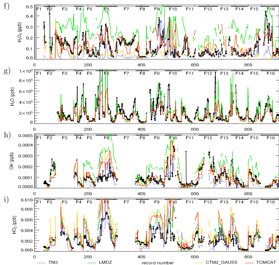
Fig. 4. (b) Continued. In panel (g) the red line showing TOMCAT is also representative of the TM3 and CTM-2 Gauss models because they all rely on ECMWF humidity fields.
