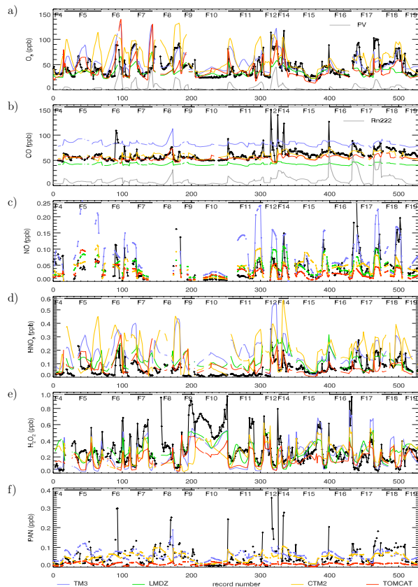
Fig. 2. Composites of PEM-Tropics A time series. Measurements at 0–35°S and 400–200 hPa (about 7.2–12 km) only. Flight numbers are indicated at the top of each panel. Black: measurements, Colors: simulations of the different models (see legend for color code). The grey line in the top panel (a) is potential vorticity (PVU) from the LMDz-INCA model, scaled by a factor of 10 to fit on the O 3 axis scale. Similarly, Rn222 (mol/1e22mol) is shown in grey in panel (b) and is displayed on the same y-axis as CO.
