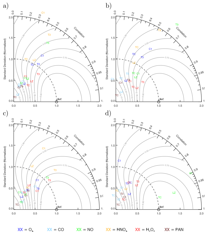
Fig. 6. Taylor diagrams of model performance for the PEM-Tropics A campaign. (a) All measurements at p < 400 hPa and between 0 and 35^\circ S latitude (same data as in Fig. 2), (b) flights 5–10 over eastern South Pacific only, (c) flights 15–18 over western South Pacific only, (d) vertical profiles at Tahiti (same data as in Fig. 3). All points of a given model are represented by a specific label: T3=TM3, C1=CTM-2 version 1, TC=TOMCAT, and LZ=LMDz-INCA. Different colors indicate different tracers (see legend at the bottom). Grey contours are isolines of model skill as defined in Eq. (1).
