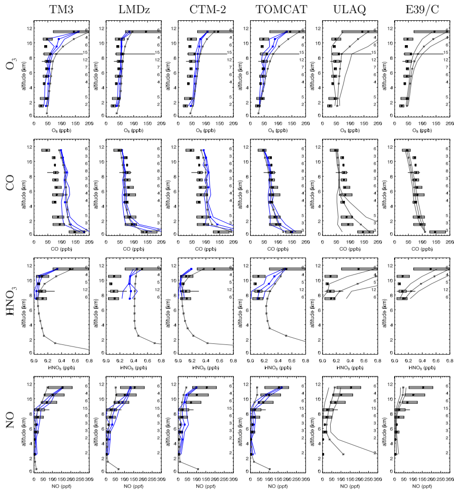
Fig. 5. (a) SONEX profiles over Shannon, Ireland. See Fig. 3 for explanation of symbols.
