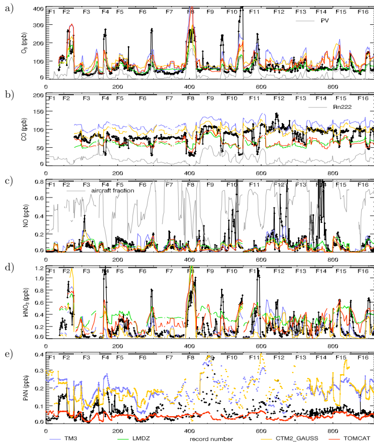
Fig. 4. (a) Composites of SONEX time series. Only measurements between 350 and 200 hPa are included. Legend as in Fig. 2. Radon values in panel (b) are from the TM3 model. The grey line in panel (c) is the fraction of NO which is contributed by air traffic emissions calculated using two TOMCAT model runs with and without including air traffic emissions (“full run”–“no aircraft”)/“full run”.
