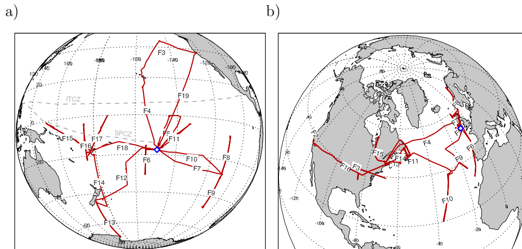
Fig. 1. Maps of (a) PEM-Tropics A, (b) SONEX measurement flights. ITCZ=Intertropical Convergence Zone, SPCZ=South Pacific Convergence Zone. Blue diamonds indicate the positions of the vertical profiles shown in Fig. 3 and Fig. 5.
