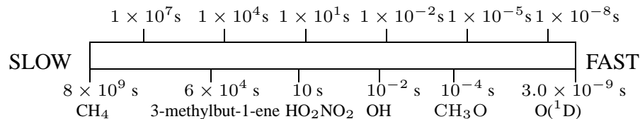
Fig. 3. Diagram showing the range of chemical lifetimes from fast to slow and examples of the lifetimes of species in the MCM.
