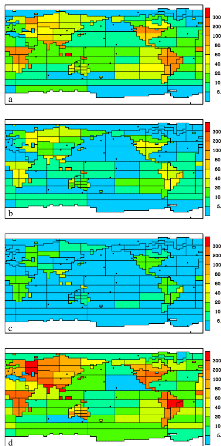
Fig. 5. Root mean square difference in source between inversion results using (a) 3 month, (b) 6 month, (c) 9 month responses and that using 12 month responses and (d) between inversion results using 12 month responses and the correct sources. The units are \text{gC m}^{-2}\text{yr}^{-1} .
