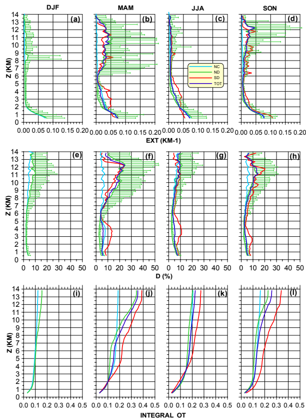
Fig. 3. Seasonal (columns) average profiles of 532 nm extinction \sigma_a (first row), depolarization ratio D (second row) and integral optical thickness OT (third row). Curve colors represent the TOT (blue), ND (green), NC (pale blue) and SD (red) records, respectively (e.g. Table 1 for synopsis). Standard deviations associated to the ND mean curves are reported for both \sigma_a and D profiles.
