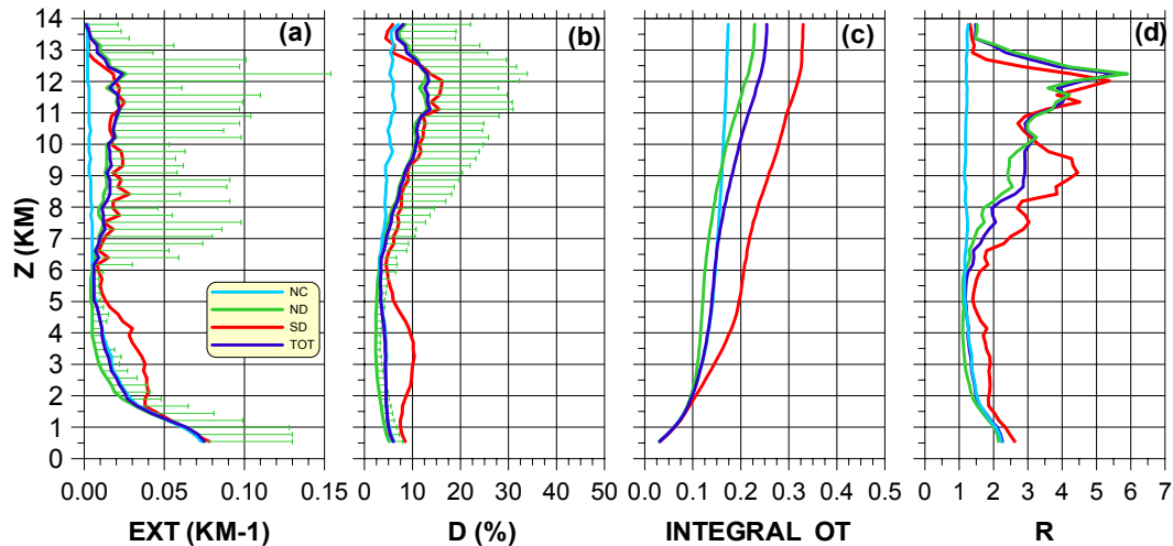
Fig. 2. Yearly average profiles (at 532 nm) of: (a) extinction \sigma_a ; (b) depolarization ratio D , (c) integral optical thickness OT(z) and (d) backscatter ratio R . Curve colors represent the total TOT (blue), no-dust ND (green), no-cirrus NC (pale blue) and Saharan dust SD (red) records, respectively (e.g. Table 1 for synopsis). Standard deviations associated to the ND mean curves are reported for both \sigma_a and D profiles.
