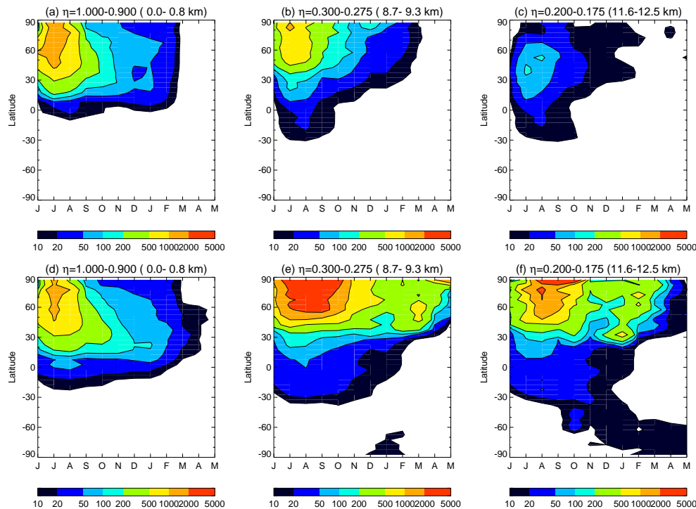
Fig. 7. Temporal evolution of the zonal mean Laki \text{SO}_4 (pptv) for Laki Lo (a–c) and Laki Hi (d–f), at three levels in the model: the surface (a, d); the upper troposphere (b, e); and the lower stratosphere (c, f). Background 1860 levels have been subtracted.
