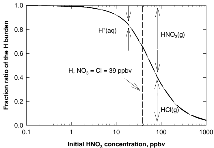
Fig. 7. Simulated distribution of the hydrogen burden for a \text{NaCl-H}_2\text{O-HNO}_3 system representative of our aerosol experiment, at equilibrium, as a function of H and \text{NO}_3 inputs. The 39.2 ppbv input for H and \text{NO}_3 (vertical dashed line) is equal to the total amount of Cl present in the system, assuming saturated sea-salt aerosols.
