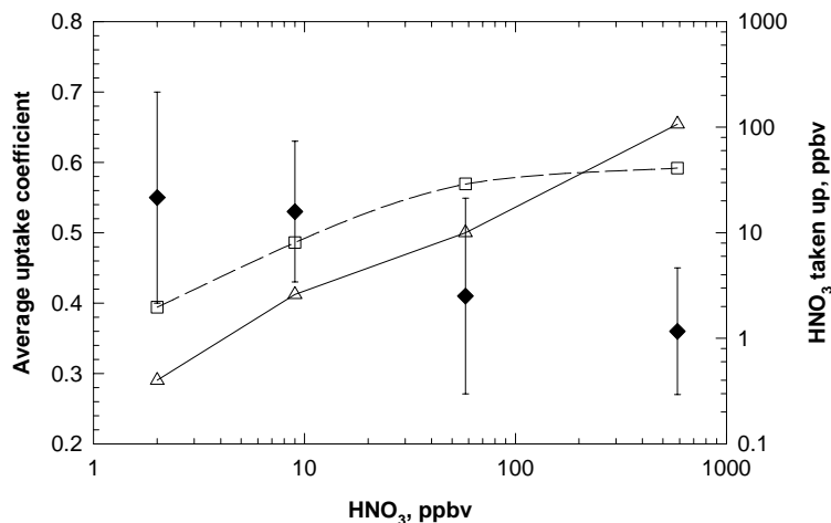
Fig. 5. Measured average uptake coefficient (plain diamonds) as a function of \text{HNO}_3 concentration (2, 9, 57 and 575 ppbv). \text{HNO}_3 taken up observed is shown for a representative reaction time of 0.7 s (empty triangles), corresponding to a flow reactor length of 20 cm. For comparison, \text{HNO}_3 taken up in the aerosol phase at equilibrium and derived from the AIM model is also shown (empty squares).
