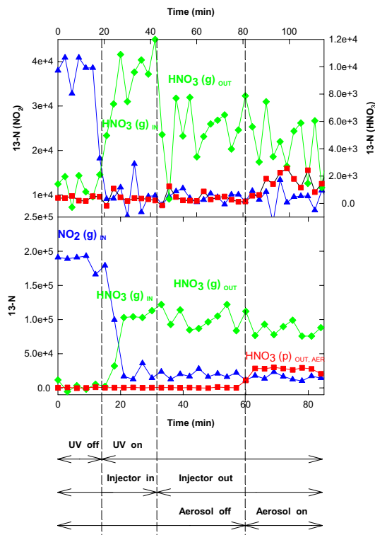
Fig. 4. On line records of \text{HNO}_3(\text{g}) (green diamonds), \text{NO}_2(\text{g}) (blue triangles), and \text{HNO}_3 attached to the particles (red squares) for a typical experiment performed at 9 ppbv (upper chart) and at 575 ppbv (lower chart) of \text{HNO}_3 present in the gas phase. Different time axis are presented for the two charts, in order to show the different steps of the protocol. Noteworthy, at low \text{HNO}_3 concentration (upper chart) the values are much more scattered, and thus a longer recording time is required to improve the statistics of the results. Also, at 9 ppbv of \text{HNO}_3 the relative decay of \text{H}^{13}\text{NO}_3 due to retention on the wall is more significant (as seen from the difference of the \text{HNO}_3 signals between injector IN and OUT, but aerosol OFF).
