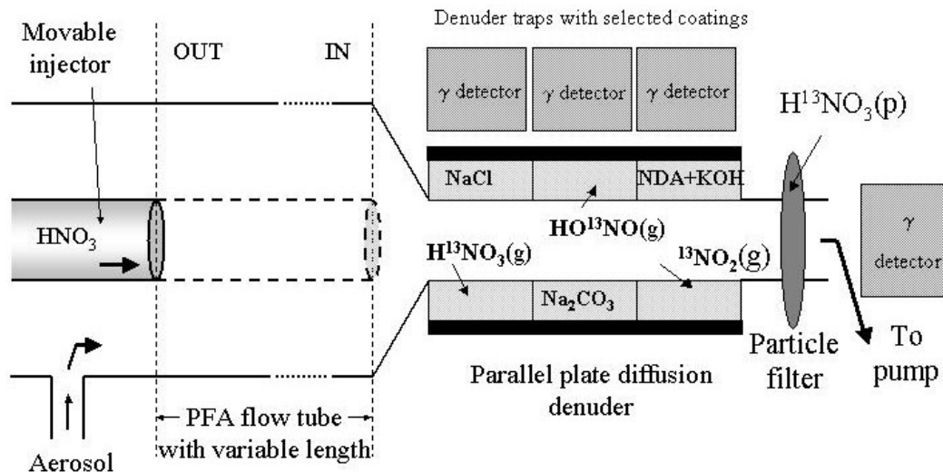
Fig. 3. Flow reactor and detection setup for gas phase molecules ( \text{NO}_2 , HONO and \text{HNO}_3 ) and for \text{HNO}_3 in particle phase ( \text{HNO}_3(\text{p}) ).
