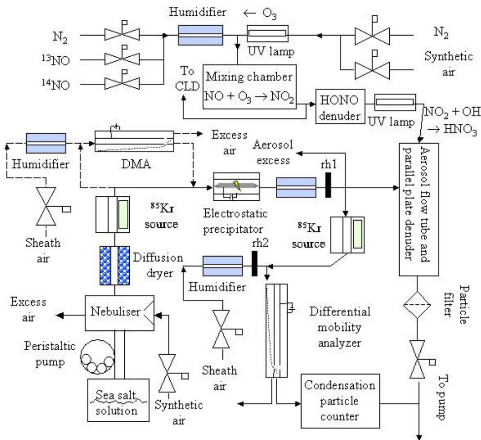
Fig. 1. Aerosol flow tube system and experimental set up to generate \text{HNO}_3 and sea-salt particles.
