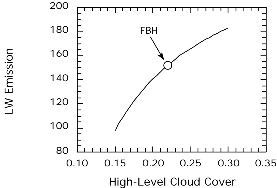
Fig. 1. Longwave emission ( \text{W m}^{-2} ) of the cloudy-moist region as a function of the fractional high-level cloud cover relative to the entire tropics. The circle represents the OLR and the high-level cloud cover derived by FBH. See the text for details.
