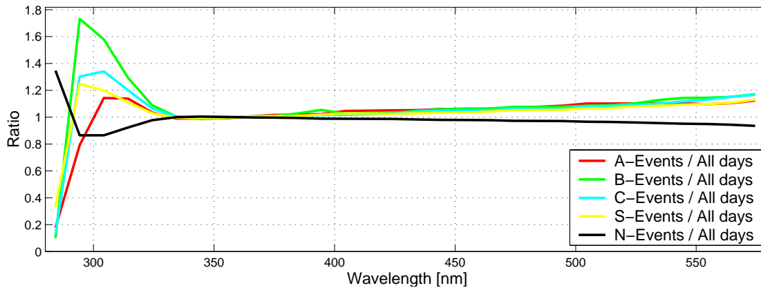
Fig. 5. (a) Average spectral solar irradiance for all event and non-event classes of 2000 and 2001; (b) Ratio of the graphs from (a) to a yearly reference graph from Eq. (4) ( \overline{E_{G,N}} ).
