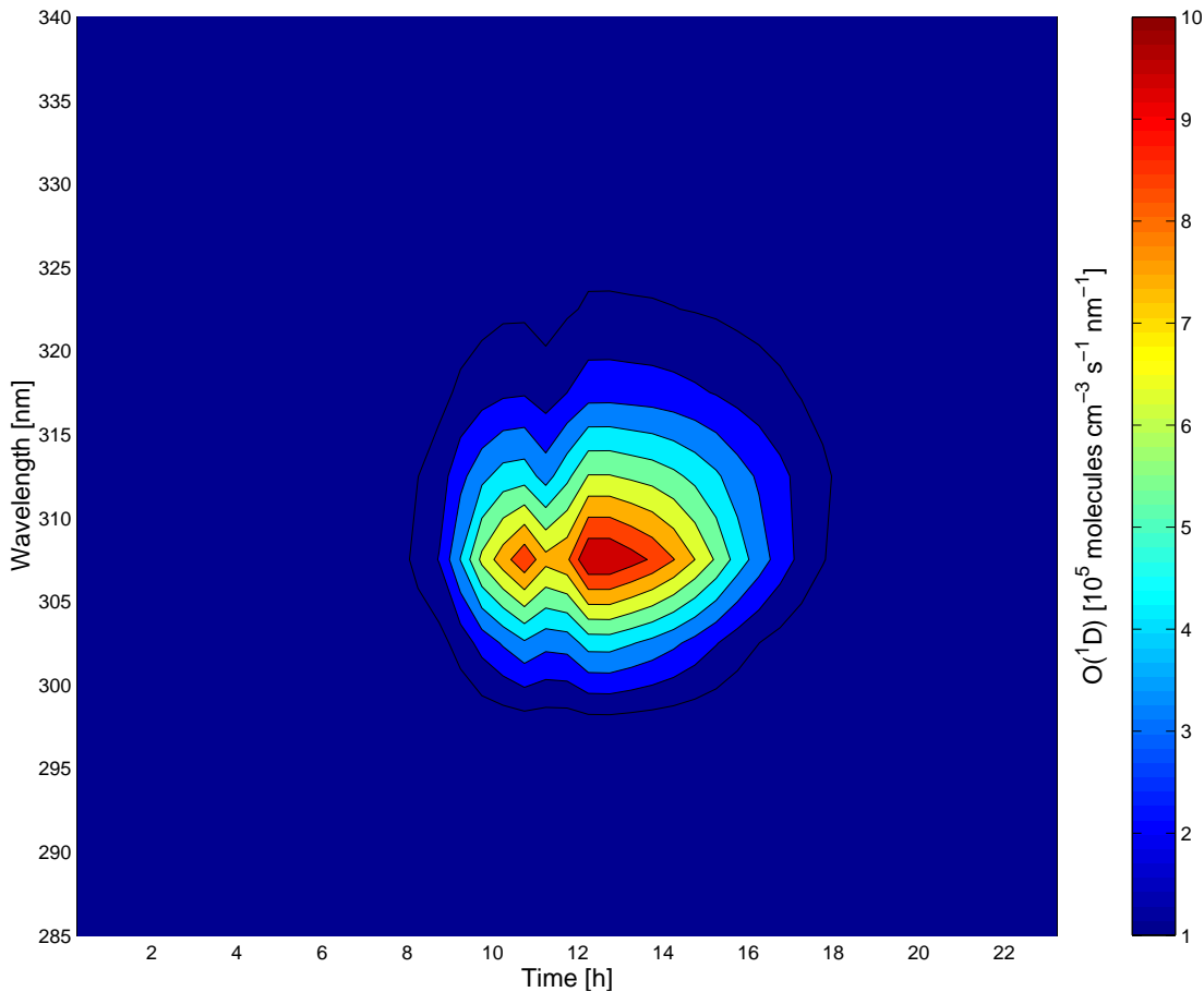
Fig. 9. Production rate of excited oxygen for 28 May 2000.
