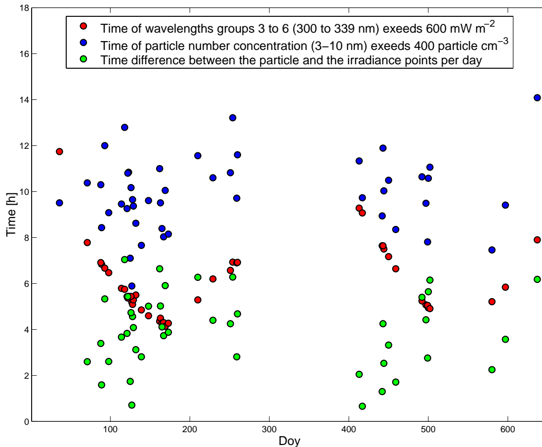
Fig. 8. Time short wavelength irradiance (300–339 nm) exceeds 600 \text{ mW m}^{-2} and particle number concentration (3–10 nm) exceeds 400 \text{ particle cm}^{-3} for A- and B-events of 2000 and 2001. Further the difference between the two explained time points are included.
