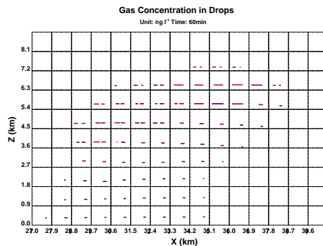
Fig. 9. Distributions of dissolved gas concentration inside drops at different locations after 40 and 60 min of simulation for the continental-sheared (blue lines) and continental-equilibrium (red lines) simulations. The solubility of the gas is equal to 10^2 \text{ mol dm}^{-3} \text{ atm}^{-1} . In one box the tick values for the abscissa are 1, 10, 1000, and 10000 \mu\text{m} , and the range for the ordinate values are from 10^{-2} to 10^4 . It should be noted that the unit in this figure is different from Fig. 10 and 11.
