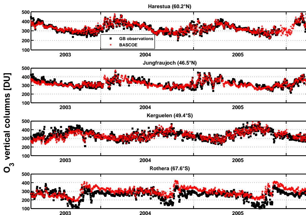
Fig. 1. Time-series of sunset stratospheric O 3 vertical columns from BASCOE analysis and ground-based UV-visible observations at 4 NDACC stations (top to bottom): Harestua, Jungfrauoch, Kerguelen and Rothera. Black squares: ground-based observations; red stars: BASCOE analysis.
