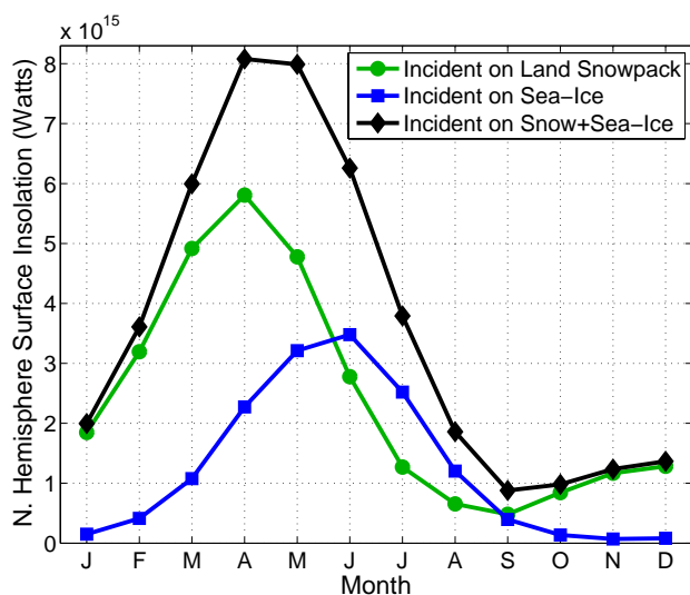
Fig. 2. Northern Hemisphere surface insolation incident upon land-based snow and sea-ice, as a function of month. Data are derived from 1990's mean annual snow and ice extent (Armstrong and Brodzik, 2005) and assimilated surface insolation (Qian et al., 2006). Insolation on land snowpack peaks in March–May, when continental snow-albedo feedback is strongest.
