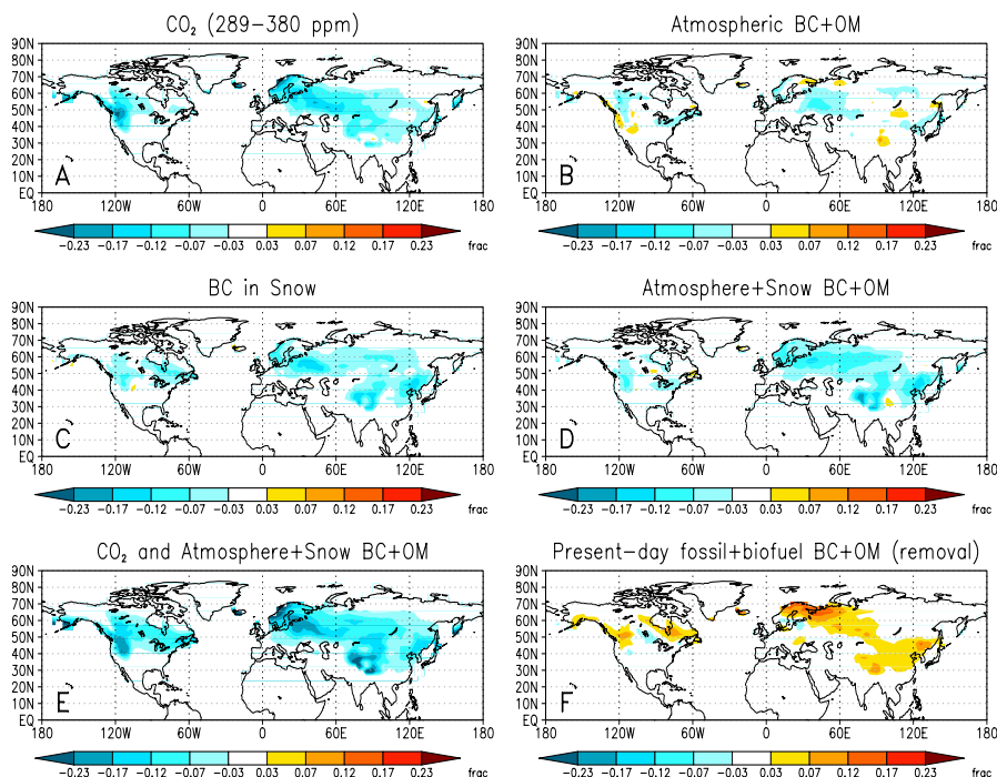
Fig. 3. Equilibrium changes in March–May snow cover fraction resulting from the following forcing mechanisms (also see Table 1): (A) CO 2 only (experiment PI2-PI1), (B) black carbon (BC) and organic matter (OM) in the atmosphere only (PI3-PI1), (C) BC in snow only (PI4-PI1), (D) BC+OM in the atmosphere and snow (PI5-PI1), (E) CO 2 and BC+OM in the atmosphere and snow (PI6-PI1), and (F) removal of all fossil fuel and biofuel emissions of BC+OM (active in the atmosphere and snow) from present climate (PD2-PD1). Continental averages of these changes are listed in Table 2.
