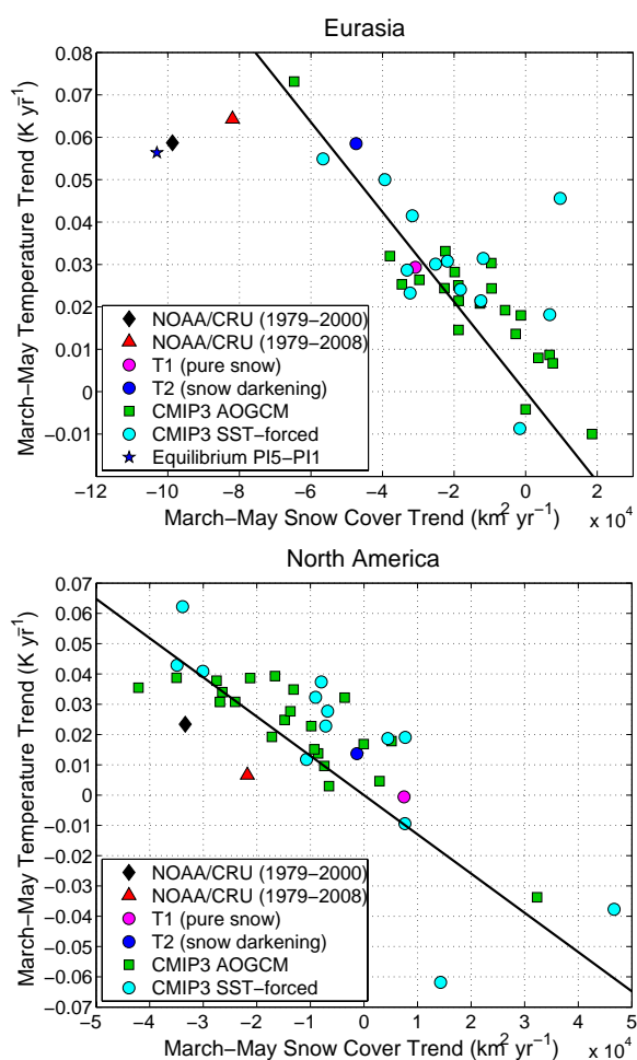
Fig. 9. 1979–2000 trends in springtime (March–May) surface temperatures (averaged over land north of 30^{\circ} N) versus corresponding trends in snow cover extent (SCE) for Eurasia (top) and North America (bottom). Data are shown for observations (CRUTEM3 temperatures and NOAA/Rutgers snow cover), AOGCM and SST-forced model data from CMIP3 (also depicted in Figs. 5 and 6), and our T1 and T2 experiments, without and with snow darkening, respectively. A datum is included showing equilibrium changes from experiment PI5–PI1 (Table 2). Because it is an equilibrium change, the position of this point is arbitrary along a line through the origin.
