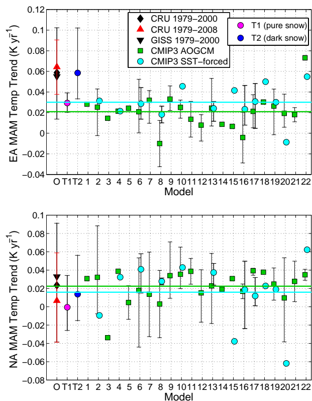
Fig. 5. Linear trends in (top) Eurasian and (bottom) North American land-averaged (north of 30^{\circ} N) March–May surface air temperatures. Observations from CRUTEM3 and NASA GISS are shown on the left-most vertical bar. 1979–2000 trends from 5-member, SST-forced ensemble experiments without (purple) and with (blue) snow darkening from black carbon and mineral dust are shown above labels “T1” and “T2”. Trends from AOGCM (green) and SST-forced (light blue) models contributing to CMIP3 and the IPCC AR4 are above labels “1–22” and described in Appendix A. Horizontal color-coded lines depict means from these two groups of models. Interval bars represent the full range of trends from all available ensemble members. Note that only 13 groups submitted SST-forced simulations, some simulations extend only through 1999, and number of ensemble members varies considerably (Appendix A). The brackets associated with observations depict 95% confidence intervals of trends, derived with the Mann-Kendall and Theil-Sen techniques.
