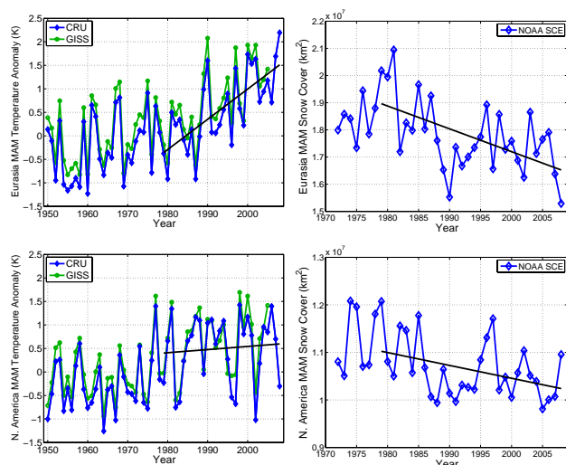
Fig. 4. Timeseries of observed springtime (March–May) temperature anomalies (averaged over land north of 30^\circ\text{N} ) and snow cover extent over Eurasia and North America. Temperature data are from CRUTEM3 (Brohan et al., 2006) and NASA GISS (Hansen et al., 2001). Anomalies are relative to different mean periods, explaining the slight offset between GISS and CRUTEM3 data. Snow cover extent is from NOAA/Rutgers (Robinson and Frei, 2000). Linear trends are shown for 1979–2008 data.
