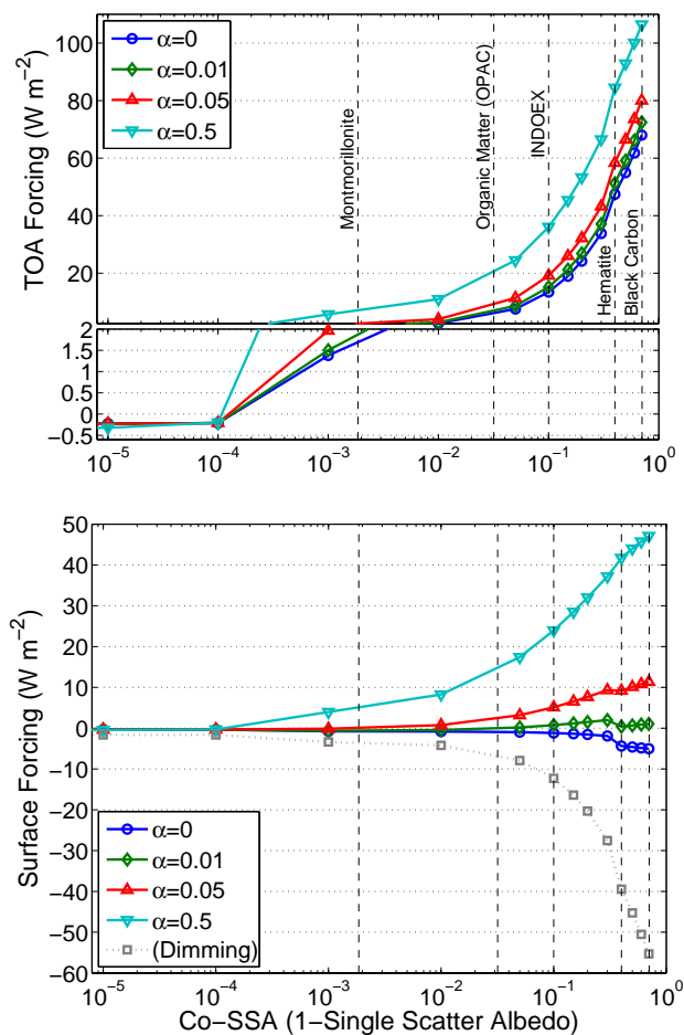
Fig. 1. Daily-mean (top) top-of-atmosphere and (bottom) surface changes in net solar power (forcing) as a function of single-scatter albedo complement ( 1\text{-SSA} ) at 500\text{ nm} . Extinction optical depth of the atmospheric aerosol is fixed at 0.2 and the environment represents a clear-sky atmosphere overlying snowpack with effective grain size of 200 \mu\text{m} on 1 April at 45^\circ\text{ N} . Curves are shown for different values of \alpha , the ratio of particle mixing ratio in snow to atmospheric column burden. Forcings represent the combined influence of particles in the atmosphere and snow. For reference, the change in downwelling surface insolation (“Dimming”) is also depicted. Vertical lines depict common SSA values of black carbon, organic matter, and that measured during the Indian Ocean Experiment (INDOEX) (Ramanathan et al., 2001). Also shown are SSA values of strongly and weakly absorbing components of dust aerosols.
