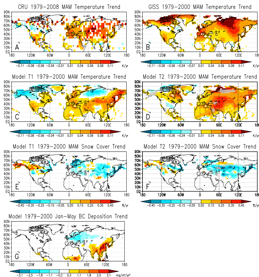
Fig. 8. Geographic distributions of springtime surface temperature, snow cover, and black carbon deposition trends. Panels depict March–May trends in (A) 1979–2008 CRUTEM3 surface temperature observations, (B) 1979–2000 NASA GISS temperature analysis, 1979–2000 ensemble-mean surface temperature from experiments (C) without snow darkening and (D) with snow darkening from deposition of black carbon and mineral dust, and snow cover fraction (E) without and (F) with snow darkening. (G) shows January–May black carbon deposition trends simulated in experiment T2, using historical emissions (Bond et al., 2007, and outlined in methods). Grey stippling in panels (D) and (F) indicates regions where trends are statistically different ( p=0.05 ) from those of the T1 ensemble.
