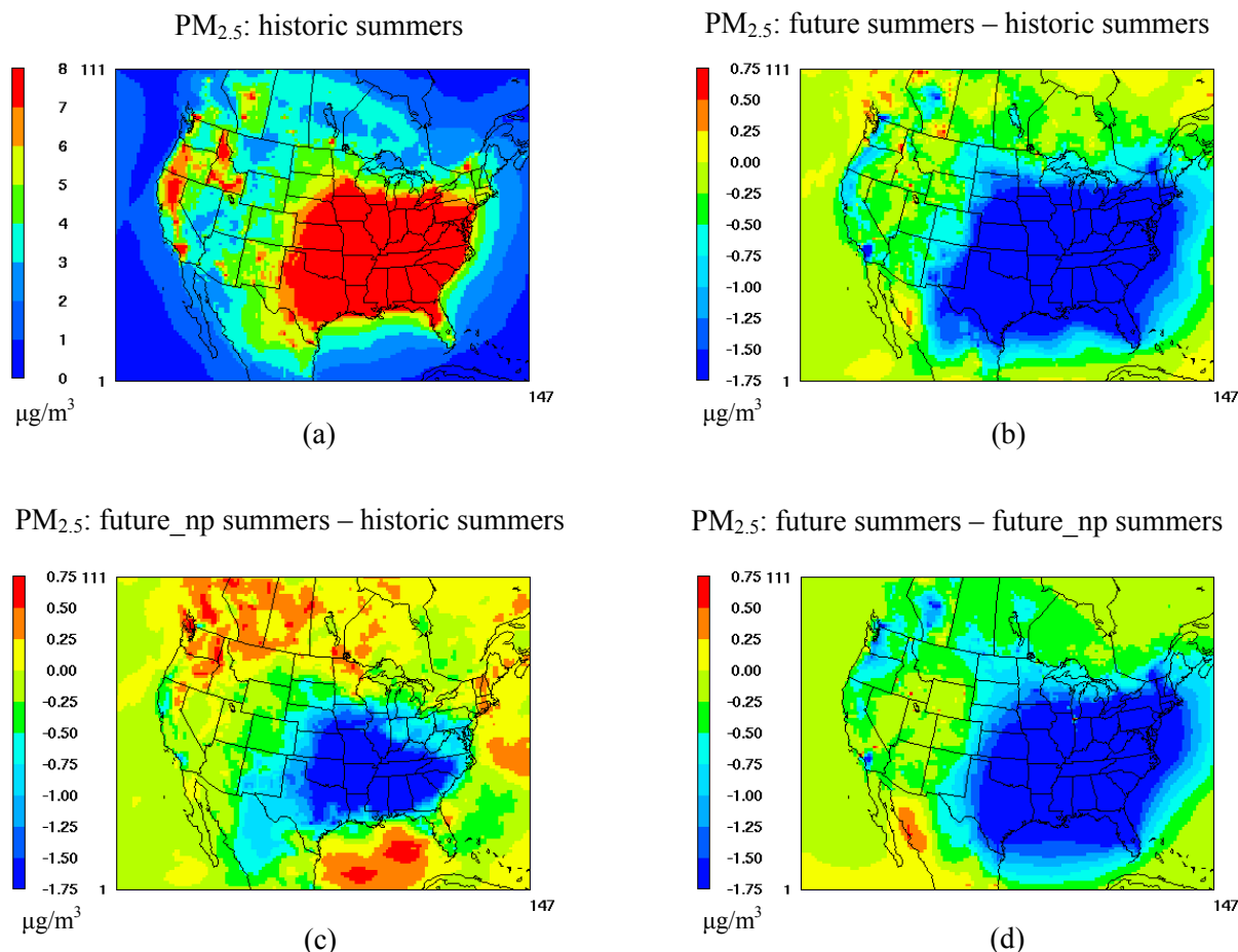
Fig. 8. (a) Three – summer – average PM 2.5 concentrations in historic years. (b) Changes in concentrations under the impact of climate change and emission controls. (c) Changes in concentrations under the impact of climate change alone. (d) Changes in concentrations under the impact of emission changes alone.
