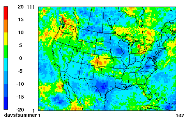
Fig. 2. Spatial distribution plot for the change in rainy days between the three historic and future summers.
