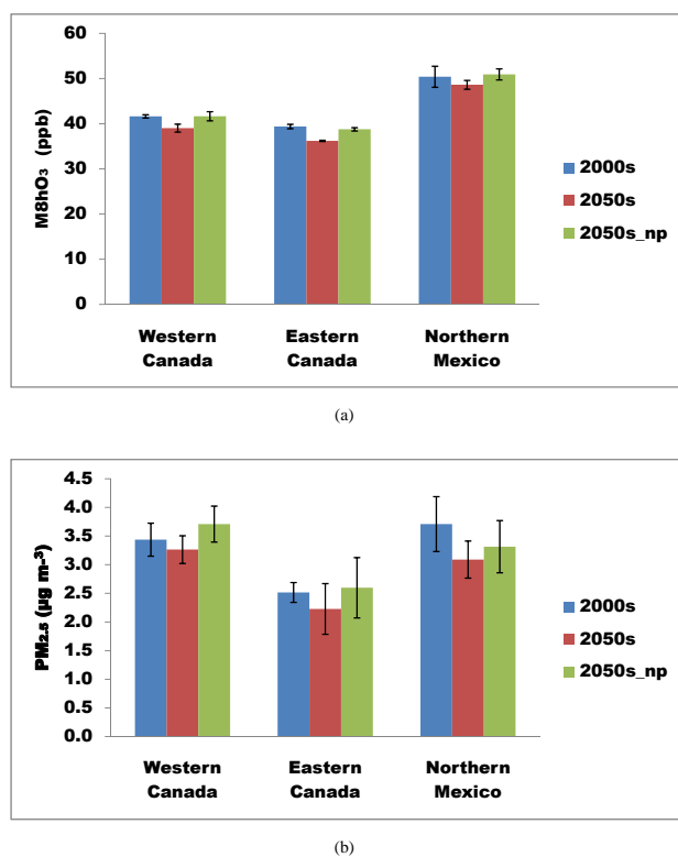
Fig. 3. (a) Mean maximum 8 h ozone concentrations (M8hO 3 ) and standard deviations for historic and future summers (b) Mean daily PM 2.5 concentrations and standard deviations for historic and future summers. (np: 2001 emission inventory and 2050 meteorology)
