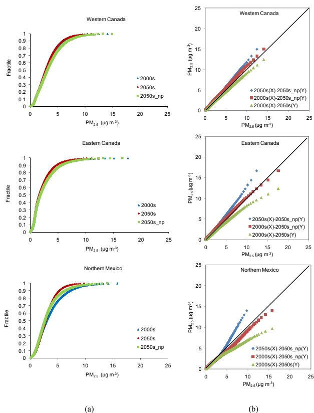
Fig. 7. Daily average PM 2.5 concentration cumulative distribution function (CDF) plots (a) for historic and future summers and the correlation (b) between the different examined cases. (np: 2001 emission inventory and 2050 meteorology)
