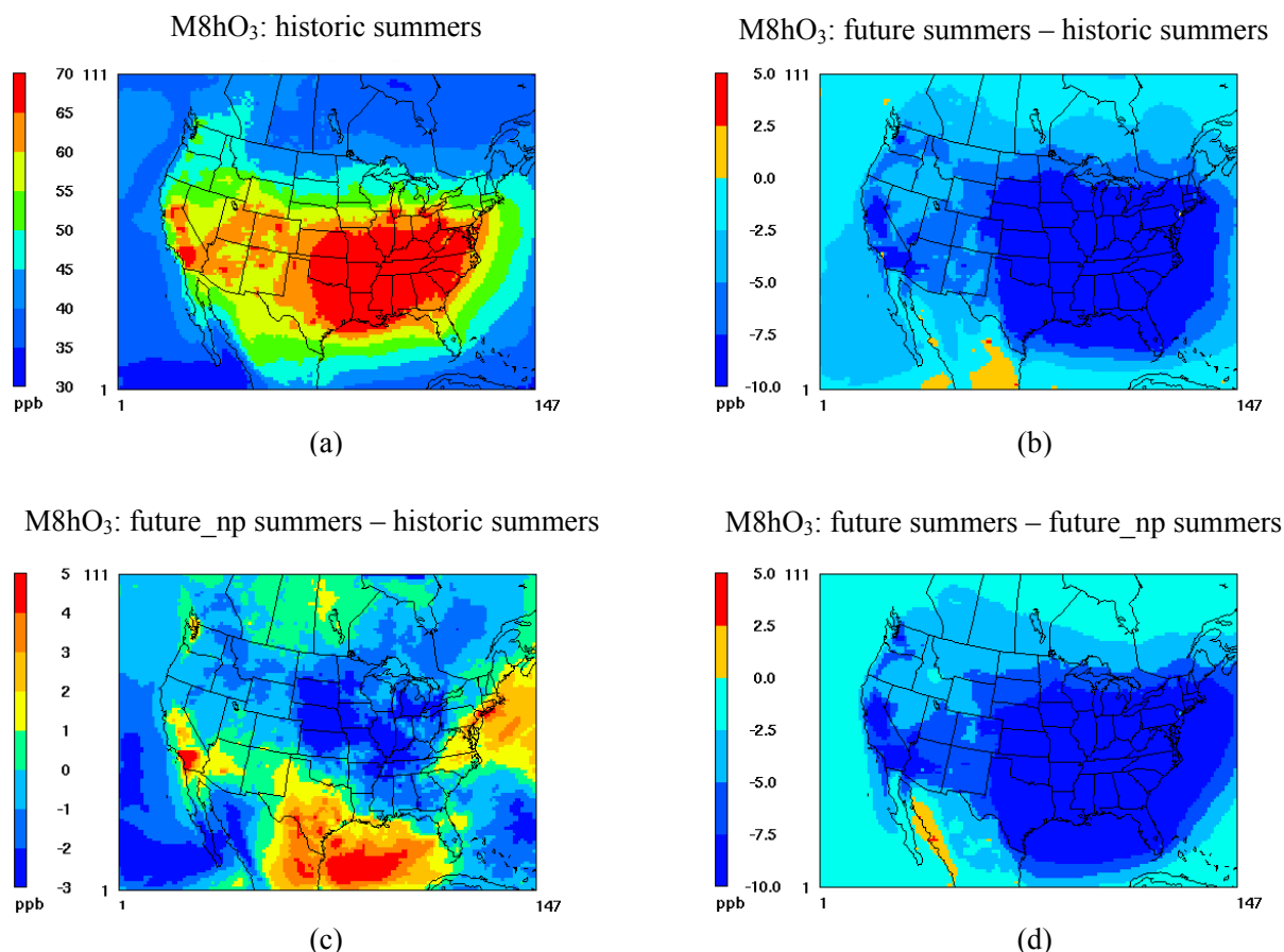
Fig. 5. (a) Three – summer – average maximum 8hr ozone concentrations in historic years. (b) Changes in concentrations under the impact of climate change and emission controls. (c) Changes in concentrations under the impact of climate change alone. (d) Changes in concentrations under the impact of emission changes alone. (np: 2001 emission inventory and 2050 meteorology)
