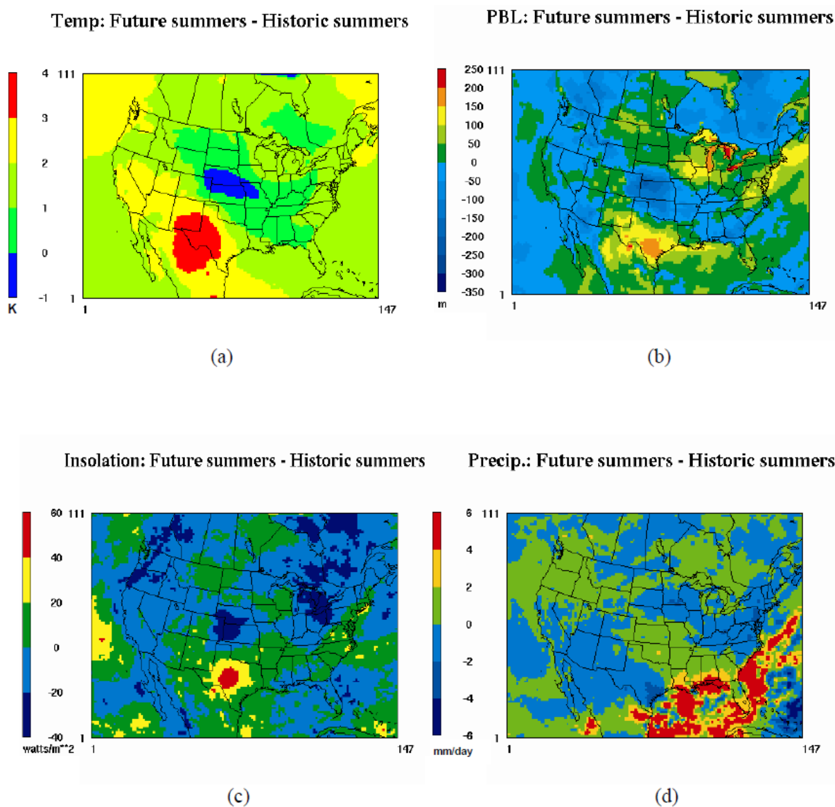
Fig. 2. Continued. Spatial distribution plots of the average changes in climatic parameters between the three historic and future summers ( a ) temperature, ( b ) planetary boundary level (PBL height), ( c ) insolation, ( d ) precipitation.
