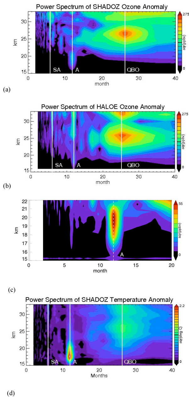
Fig. 6. Power spectrum of (a) SHADOZ and (b) HALOE tropical ozone mixing ratio anomaly field ( \text{ppbv}^2 ) versus period in months, (c) same as (a) but a close-up of the annual amplitudes, and (d) SHADOZ temperature anomaly ( ^{\circ}\text{C}^2 ). White vertical lines mark the semi-annual, annual, and the QBO periods and are noted by “SA”, “A”, and “QBO”, respectively.
