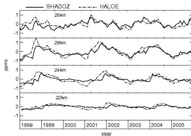
Fig. 3. Monthly time series of ozone anomalies (ppmv) for SHADOZ (solid) and HALOE (dashed) at various altitude levels that are limited to the HALOE vertical resolution (2 km).
