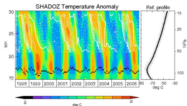
Fig. 4. Monthly time series curtain plot of ozonesonde temperature anomalies (degree C) with overlaid lined contours of QBO wind shear (m/s/km) in white, as in Fig. 1. Filled black diamonds are the mean monthly cold point tropopause heights. Right panel is a plot of the reference temperature profile. Gray shading indicates the one-sigma deviation from the mean.
