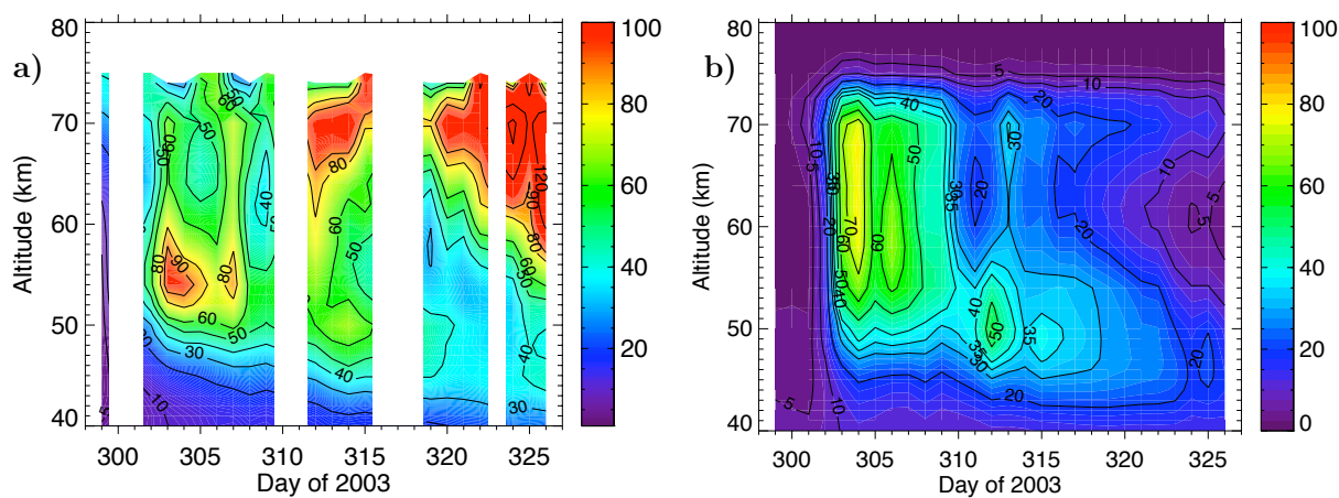
Fig. 7. Time series of NO 2 abundances (in ppbv) after the solar proton events of October–November 2003 for the Northern Hemisphere polar cap (70–90° N) at nighttime conditions as measured by MIPAS (a) and modeled by the Canadian Middle Atmosphere Model (CMAM) (b) with application of the averaging kernels of MIPAS retrievals. The vertical white bands in panel (a) represent days with no processed data.
