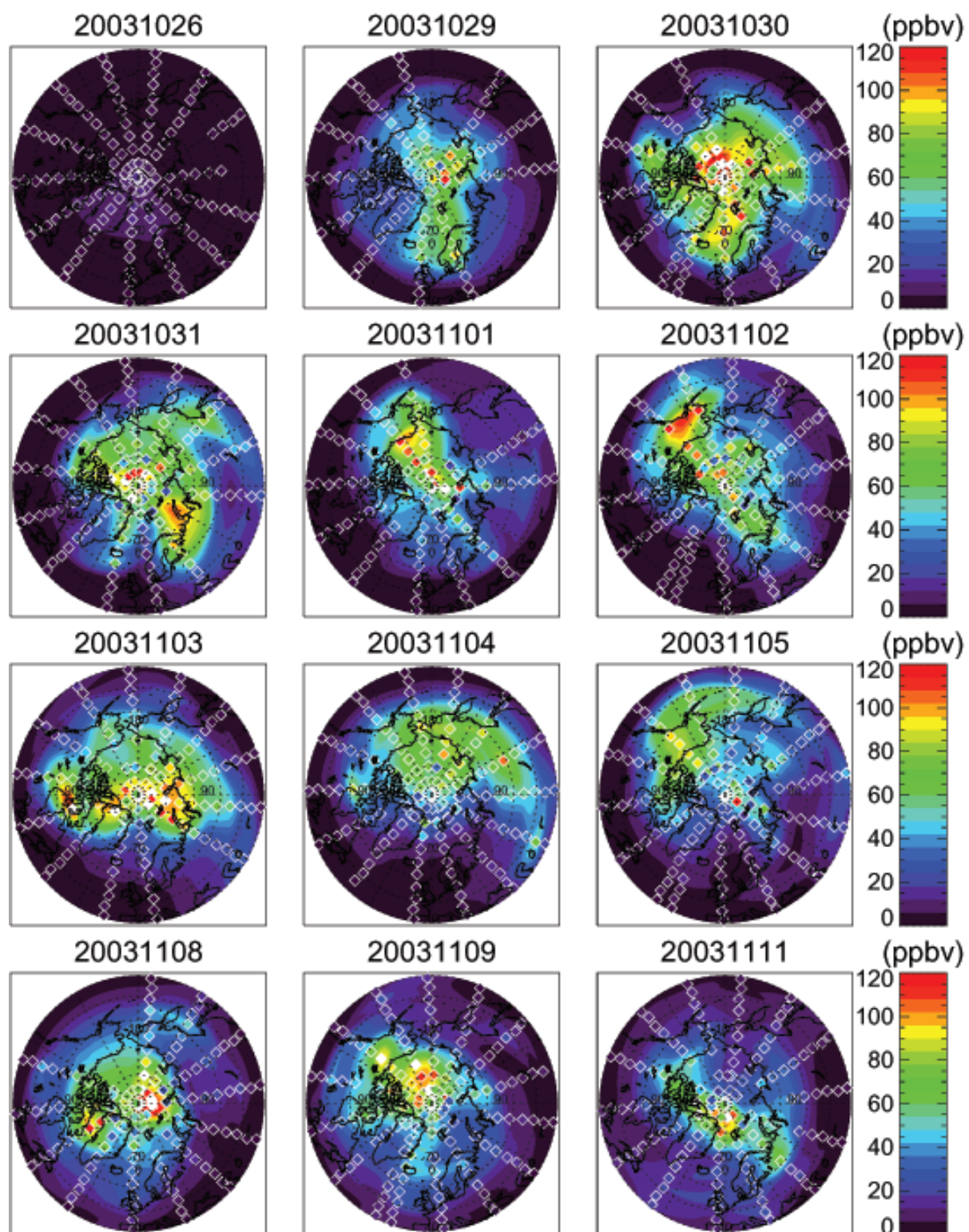
Fig. 2. As Fig. 1 but for NO 2 .
