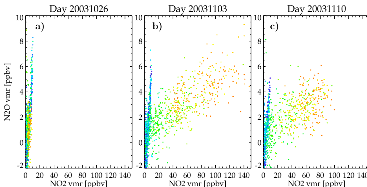
Fig. 3. Correlation plots of N 2 O versus NO 2 for the Northern Hemisphere for days 26 October (before the SPE) and 3 and 10 November (after the SPE). The color code indicates the latitudes, ranging from the equator (dark blue) until North pole (orange). The data included comprise altitudes from a potential temperature of 2000 K (~40 km) to 3000 K (~60 km). Only nighttime data is included.
