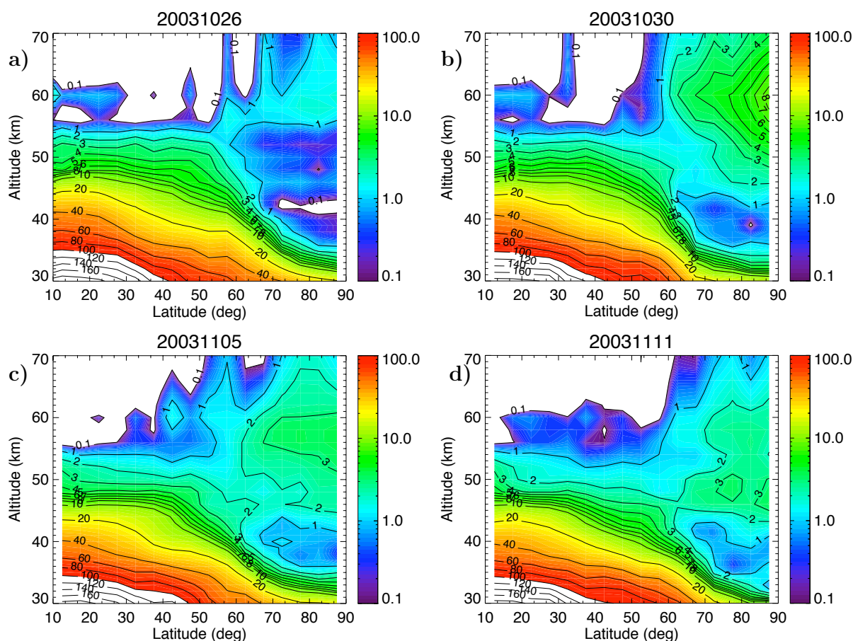
Fig. 4. Zonal mean cross sections of N 2 O (in ppbv) in the Northern Hemisphere for the days 26 and 30 October ( a, b ) and 5 and 11 November ( c, d ) 2003 measured in nighttime conditions. The enhancement of N 2 O at high latitudes above 40 km is evident in panels b–d. White areas at highest altitudes represent MIPAS measurements with no information and those at the lowest altitudes near the tropics denote values outside of the color scale range.
