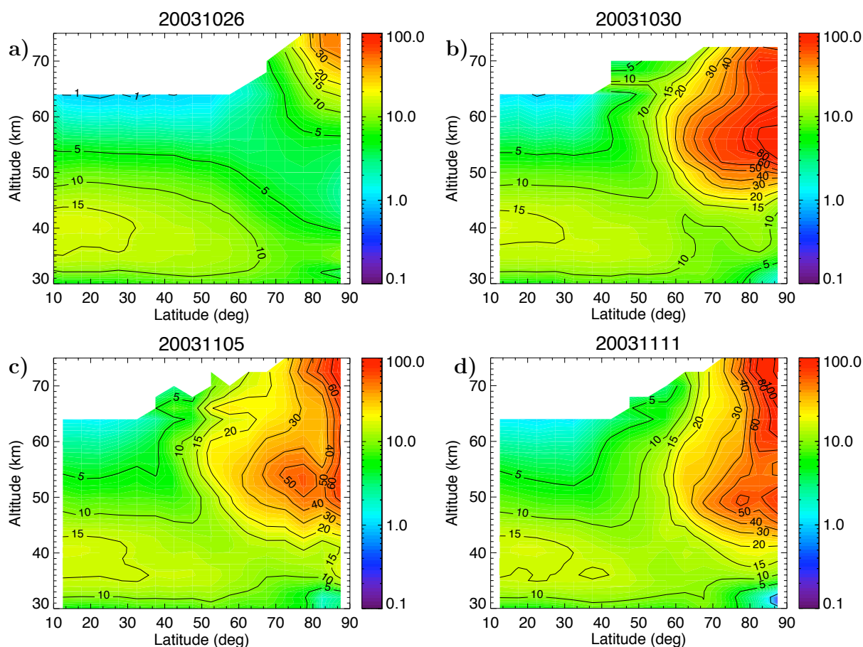
Fig. 5. As Fig. 4 but for NO 2 .
