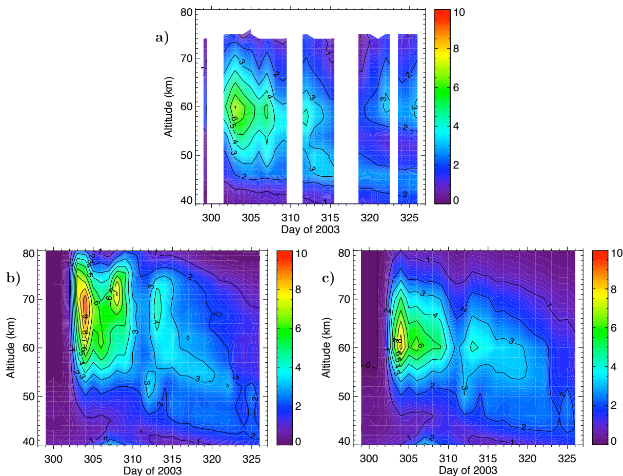
Fig. 6. Time series of N 2 O abundance (in ppbv) after the solar proton events of October–November 2003 for the Northern Hemisphere polar cap (70–90° N) during nighttime conditions. (a) MIPAS measurements; where white areas at highest altitudes represent MIPAS measurements with no information and the vertical white bands represent days with no processed data. Lower panels: Simulations by the Canadian Middle Atmosphere Model without (b) and with (c) application of the averaging kernels of the MIPAS retrievals.
