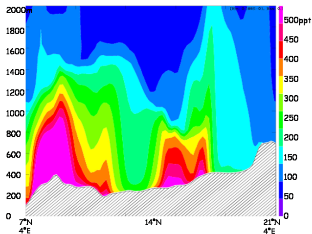
Fig. 8. Vertical cut of \text{NO}_x concentrations in ppt (4.0° E, from 7 to 21° N), ALLNOX simulation, from 0 to 2000 m. 2006/08/06 15:00 UTC
