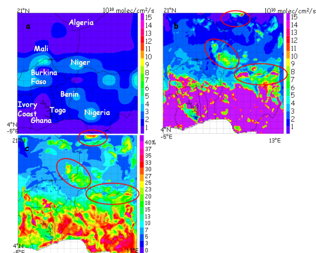
Fig. 2. (a) Biogenic NO emissions from soil ( 10^{10} \text{ molec cm}^{-2} \text{ s}^{-1} ) in August, provided by GEIA database, from Yienger and Levy (1995) inventory, (b) biogenic emissions from soils ( 10^{10} \text{ molec cm}^{-2} \text{ s}^{-1} ) provided by the on line ANN algorithm, 2006/08/06 15:00 UTC, and (c) soil moisture (%), 2006/08/06 15:00 UTC. Red circles highlight the correspondence between strong moisture and high emissions.
