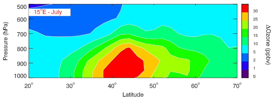
Fig. 5. Vertical cross-section at 15° E of the difference in model ozone (ppbv) in July between RUN1 and RUN2.
