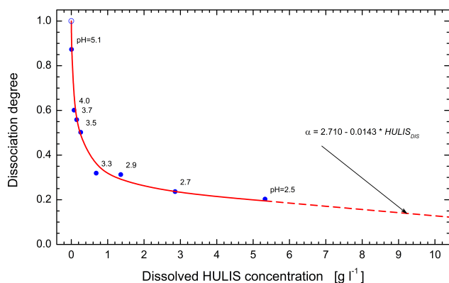
Fig. 4. Dissociation degree ( \alpha ) of pure HULIS solution with different dissolved HULIS concentration ( \text{HULIS}_{\text{DISS}} ). Solution pH values measured are also indicated. The connecting curve represents an eye-guide only.
