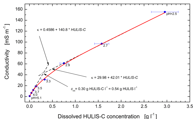
Fig. 3. Electrochemical conductivity ( \kappa ) of pure HULIS solutions with different dissolved carbon concentration ( \text{HULIS-C} ). The connecting curve represents an eye guide only. The limiting linear lines (dashed lines) and their analytical expression far before and after the intersection-point, the concentration for the intersection-point, and the solution pH values measured are also indicated.
