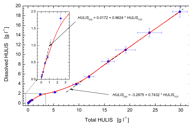
Fig. 2. Dependence of the dissolved HULIS concentration ( \text{HULIS}_{\text{DIS}} ) on the total HULIS concentration ( \text{HULIS}_{\text{TOT}} ) in aqueous samples. The range of small concentrations is also displayed in an insert. The connecting curves represent eye guides only. The limiting linear lines (dashed lines) and their analytical expressions are also shown.
