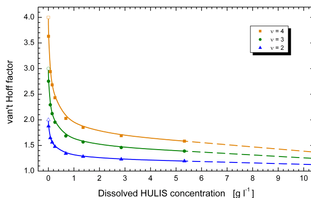
Fig. 5. Concentration dependence of the van't Hoff factor for pure HULIS solution for stoichiometric dissociation numbers of 2, 3 and 4.
