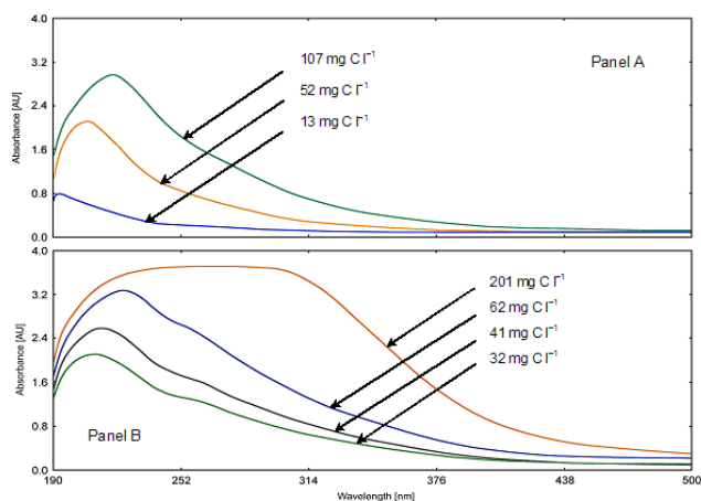
Fig. 1. UV/Vis spectra of atmospheric HULIS (Panel A) and standard SRFA (Panel B) aqueous solutions with different concentrations.
