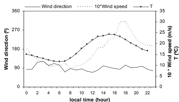
Fig. 5. Mean hourly temperature, wind direction (vectorial mean) and wind speed recorded at T0 from 1st to 26th March 2006.
