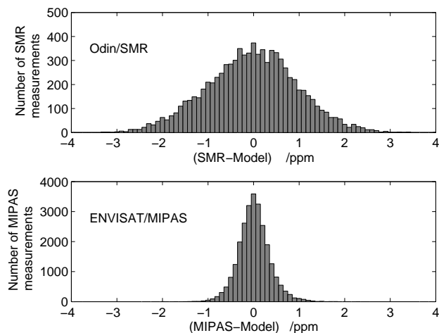
Fig. 4. Observations minus model background on the 475 K potential temperature level. All observations included in the histograms were made north of 30^\circ N during January, February and March of 2003.
