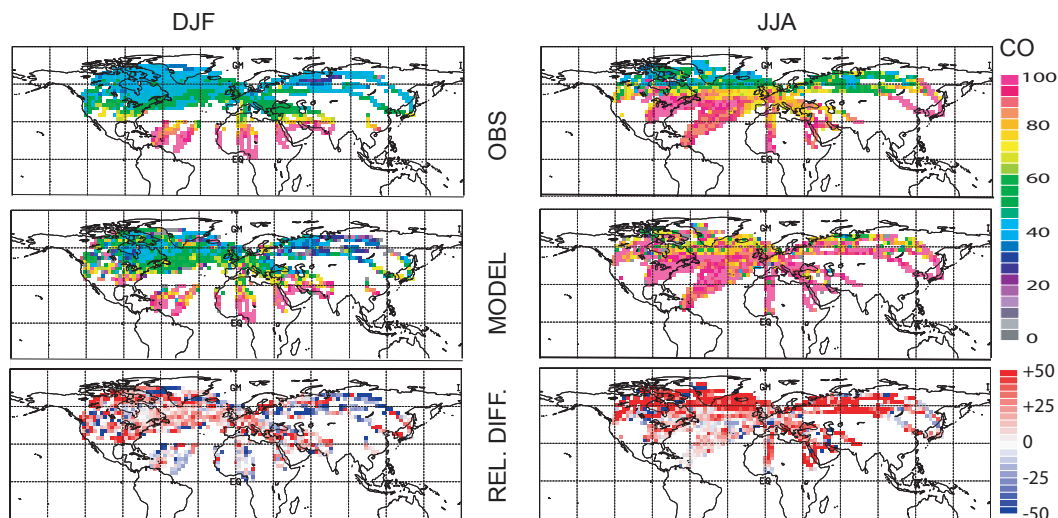
Fig. 4. Distribution of CO mixing ratio (ppbv) in 3-D boxes ( 2.8^{\circ} \times 2.8^{\circ} along the horizontal, 340–350 K potential temperature layer), as seen by MOZAIC (top panels), simulated by MOCAGE-Climat (T42 experiment, middle panels) and relative differences ( 100 \times (\text{MOCAGE} - \text{MOZAIC}) / \text{MOZAIC} ) for winter (DJF, left) and summer (JJA, right) of the 2000/2004 period.
