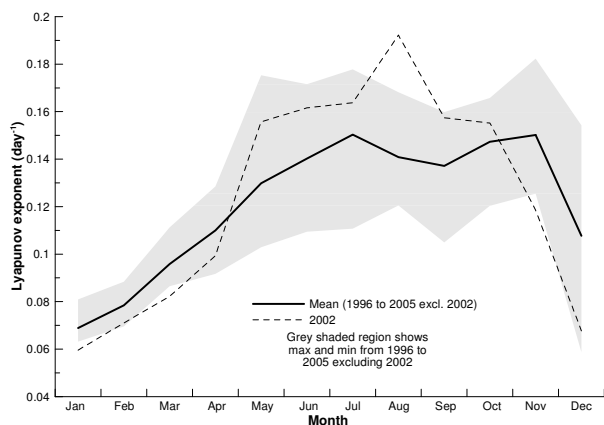
Fig. 4. Lyapunov exponents averaged over 60^{\circ} S to 90^{\circ} S at 650 K for 2002 (dashed line). The 10-year mean 1996 to 2005 (excluding 2002) is shown as a solid line together with the range of values over this time period (grey shaded region).
