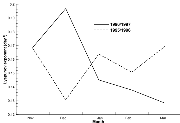
Fig. 5. Lyapunov exponents averaged over 60^{\circ} N to 90^{\circ} N at 450 K for the northern winters 1995/96 (dashed line) and 1996/97 (solid line).
