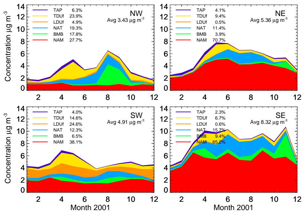
Fig. 7. Monthly and regional average of surface aerosol fine mass in NW, SW, NE, and SE (domain in Fig. 3) in the U.S. from different origins: TAP, transported air pollutants from outside North America; \text{TDU}_f , imported fine-dust from outside North America; \text{LDU}_f , local fine-dust; NAT, natural (biogenic and volcanic); BMB, biomass burning; NAM, North American pollution.
