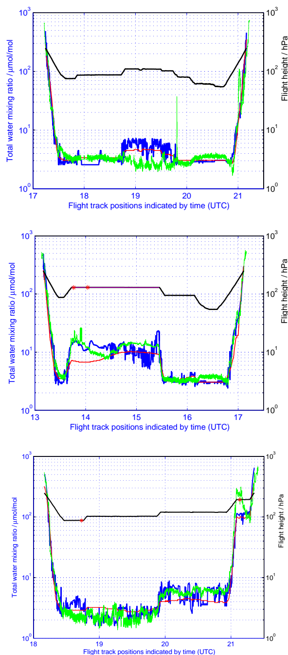
Fig. 6. Water vapour mixing ratios ( \mu\text{mol/mol} ) by FISH measurements (green), ECMWF-analysis reconstructions (red), and LACM reconstructions (blue), using 10-day backward trajectories released from the flight tracks flown by the high-altitude aircraft Geophysica on the 5, 8, 18 February 2005 (from top to bottom), for the TROC-CINOX field campaign in Brazil. The flight heights are also shown in black. In the middle panel, the magenta line shows where the trajectories in Figs. 2 and 5 ended, while the two red stars correspond to Fig. 3. In the bottom panel, the two red stars correspond to Fig. 1.
