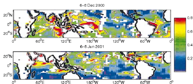
Fig. 10. Fraction of observations (colour scale) between latitude 30° N and 30° S and longitude 0 to 360° E during the 6–8 December 2000 (upper panel) and 6–8 June 2001 (lower panel) periods whose optical depth \tau exceeded 0.02. White indicates less than 1000 measurements in the box. Gray contours indicate the 30% frequency contour for \tau > 0.03 . (Reproduction of Fig. 2 of Dessler and Sherwood, 2003, by the courtesy of the authors and AMS)
