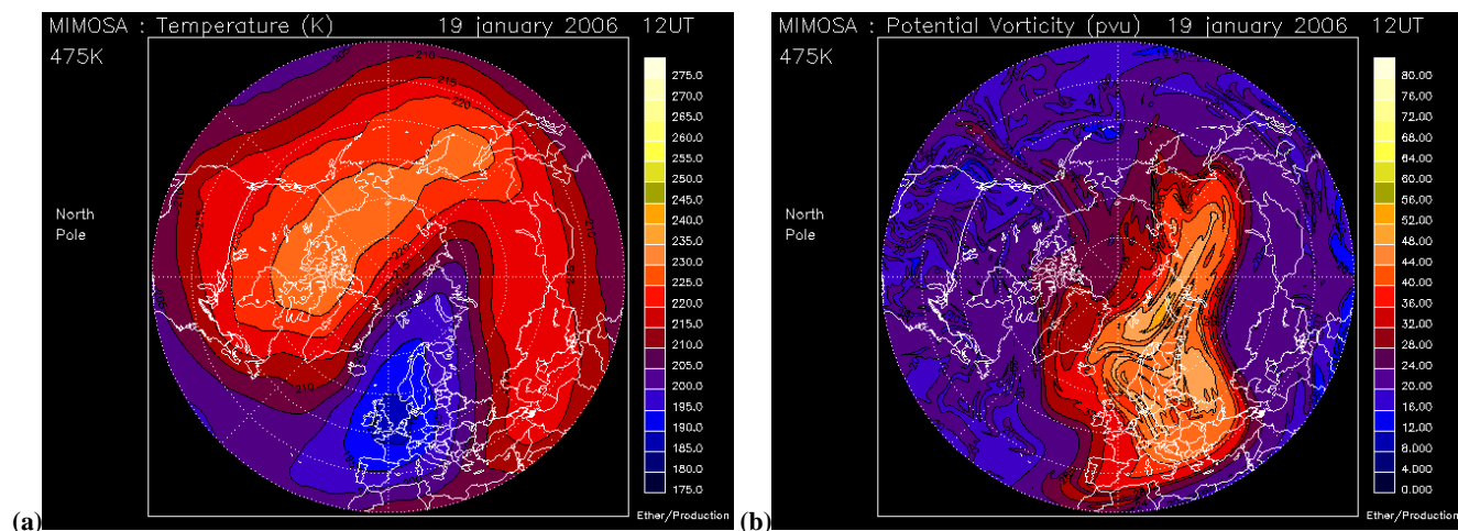
Fig. 3. Maps of the temperature and Vorticity on 19 January at 12:00 UT. Temperatures are given in K (a) and Potential Vorticity is given in PVU (b) on the 475 K isentropic level. High-resolution potential vorticity is calculated with the advection model MIMOSA (Hauchecorne et al., 2002) driven by ECMWF (European Centre for Medium-Range Weather Forecast) wind field, while temperature field are also deduced from ECMWF analysis. The edge of the polar vortex edge is usually defined as the region of maximum PV gradients that correspond approximately to the 36 PVU contour on the figure. Maps are available on http://ether.ipsl.jussieu.fr/ for previous and past days.
