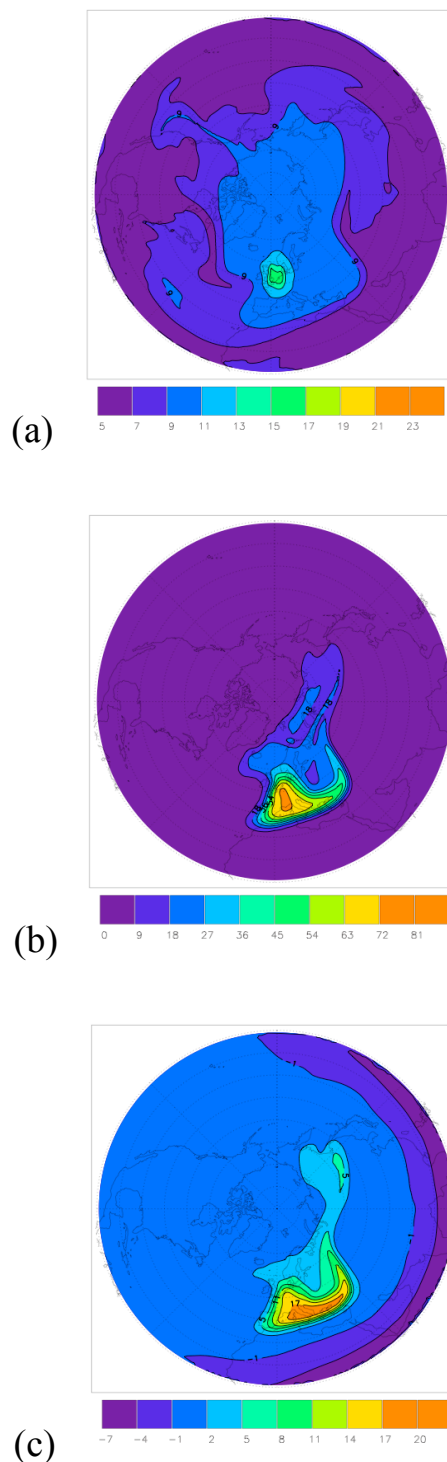
Fig. 4. Maps of PSC, Chlorine activation, and associated ozone loss estimated with numerical simulations. Model-calculated maps of (a) PSC surface area (in 10^{-9} cm 2 /cm 3 ), (b) ClO x /Cl y ratio (active Chlorine species = Cl, ClO, Cl 2 , Cl 2 O 2 , HOCl) and (c) cumulative ozone loss (in ppb over the previous 12 h) at 462 K, on 19 January at 12:00 UT.
