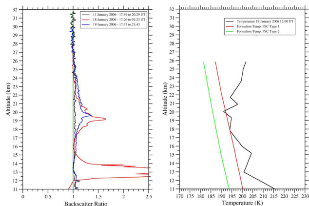
Fig. 1. Lidar backscatter ratio and collocated radiosonde temperature profile. (a) Lidar backscatter ratio profiles measured at the Observatory of Haute-Provence on 11 January 2006 showing typical background aerosol signature and on 18 and 19 January.
