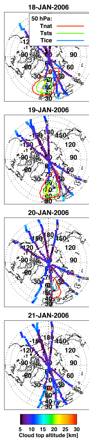
Fig. 2. PSC top heights derived from MIPAS/Envisat observations on 18 to 21 January 2006. PSCs appear as green, yellow and orange squares indicating PSC top altitudes between 18 and 25 km. Red, green and blue contour lines indicate PSC threshold temperatures at 50 hPa as deduced from ECMWF analyses for respectively Nitric Acid Trihydrate (NAT), Supercooled Ternary Solution (STS) and ice.
