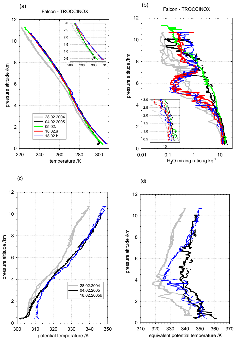
Fig. 17. Vertical profiles (1 s values) for temperature (a), H 2 O mixing ratio (b), potential temperature Θ (c), and equivalent potential temperature Θ e (d) derived from Falcon measurements for tropical (4–5 February 2005) and subtropical (28 February 2004 and 18 February 2005) air masses. In (a) and (b) the lower part of the profile (up to 3 km) is shown enlarged in the insets.
