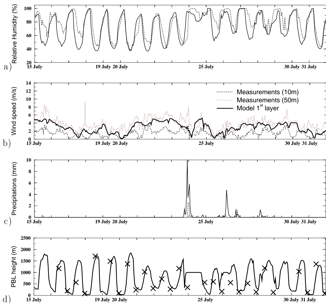
Fig. 7. Time series of meteorological variables (relative humidity (a), wind speed (b) and precipitations (c)) simulated by the model (full line) and observed at Saclay site (dotted line) from 15 July to 1 August 2000. The comparison of PBL height (d) calculated by the model (full line) and observed by Trappes radiosoundings (crosses) twice a day at 00:00 and 12:00 UTC is also presented. The 24 and 26 July undergo instable, cloudy weather conditions.
