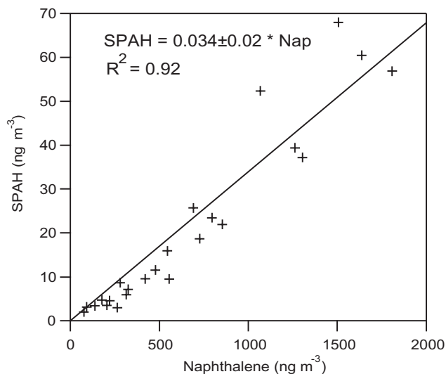
Fig. 5. SPAH versus naphthalene (gas-phase) concentrations. The uncertainty in SPAH is estimated to be 20%. Naphthalene was collected on Tenax in replicate with an average relative standard deviation of 8%.
